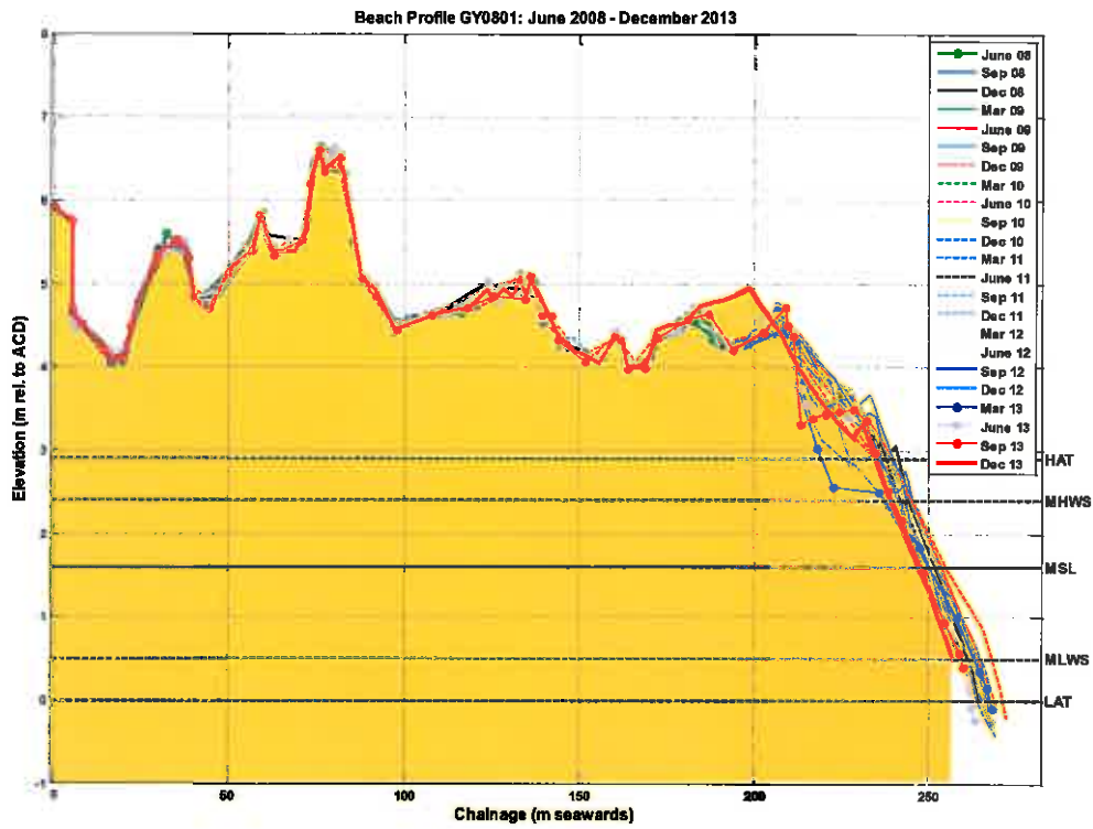
Figure B.2: Beach level surveys of profile GY0801
