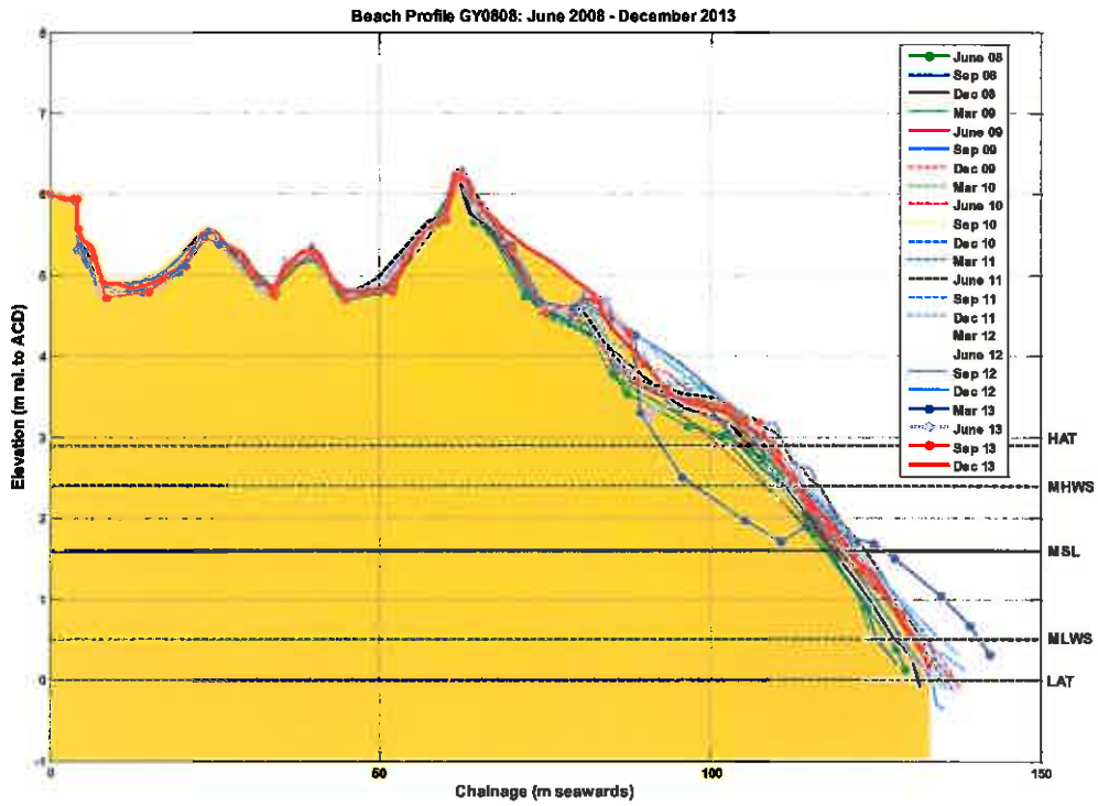
Figure B.9: Beach level surveys of profile GY0808
