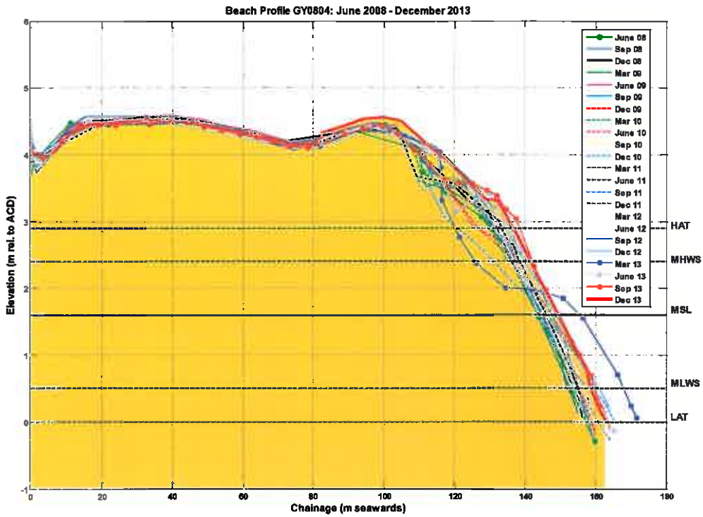
Figure B.5: Beach level surveys of profile GY0804
