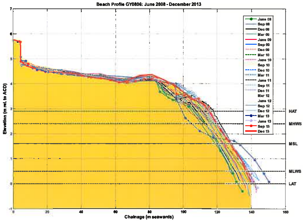
Figure B.7: Beach level surveys of profile GY0806
