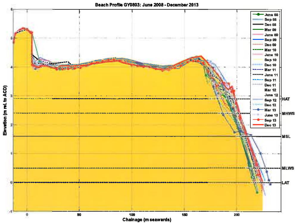
Figure B.4: Beach level surveys of profile GY0803
