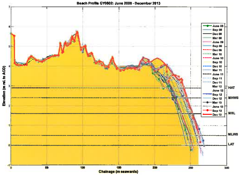
Figure B.3: Beach level surveys of profile GY0802
