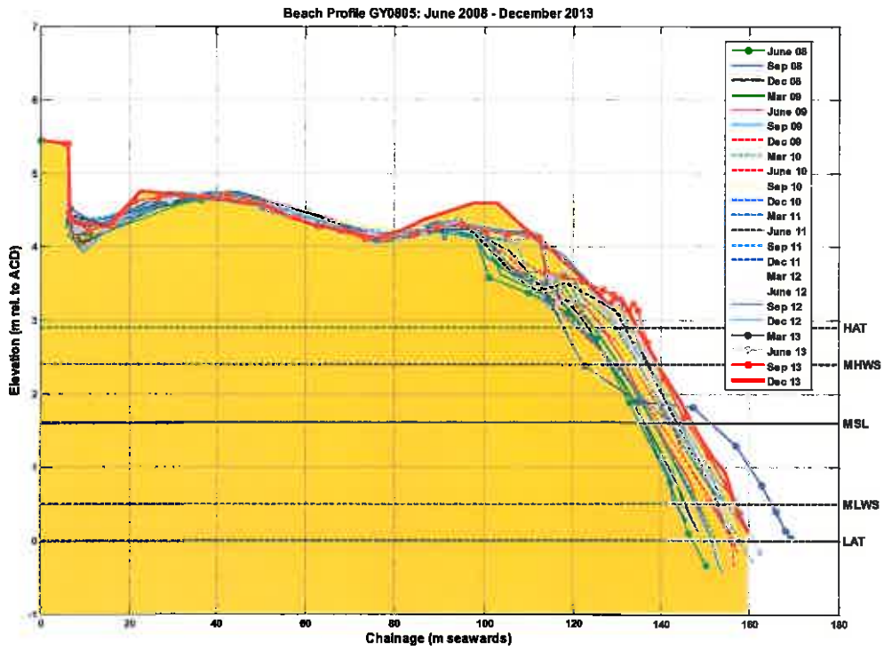
Figure B.6: Beach level surveys of profile GY0805
