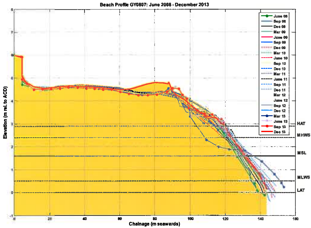
Figure B.8: Beach level surveys of profile GY0807
