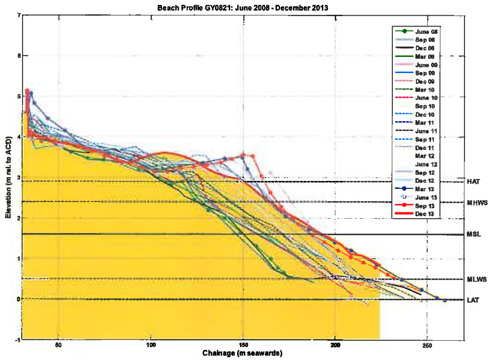
Figure B.17: Beach level surveys of profile GY0821
