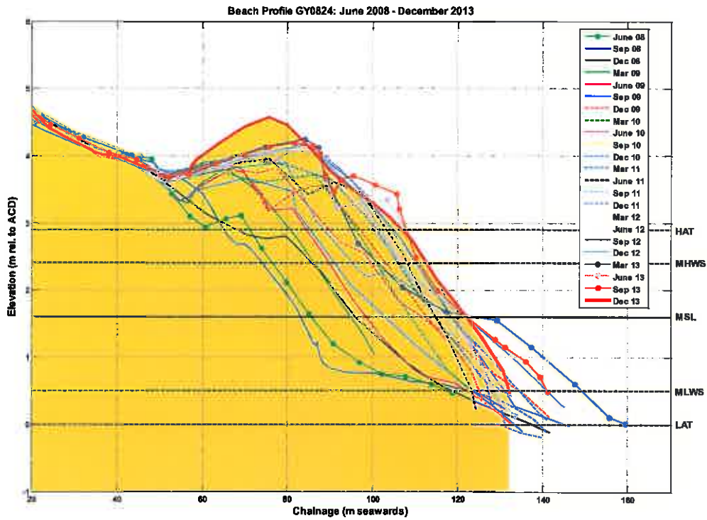
Figure B.20: Beach level surveys of profile GY0824
