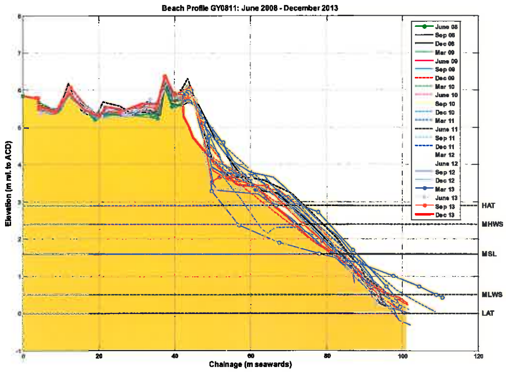
Figure B.12: Beach level surveys of profile GY0811
