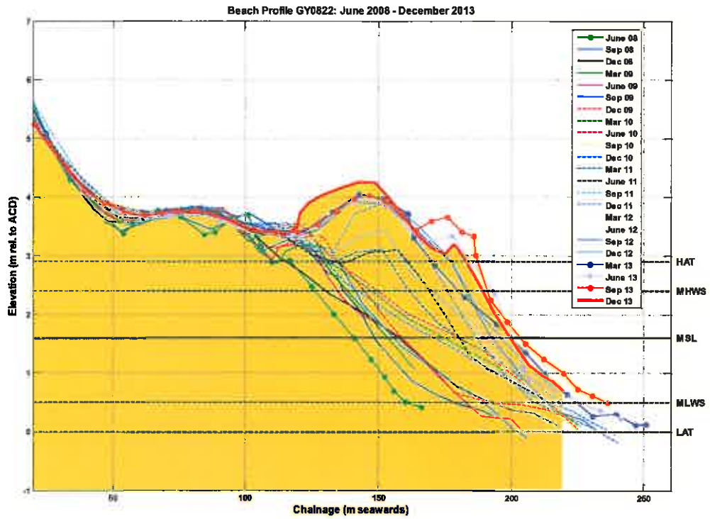
Figure B.18: Beach level surveys of profile GY0822
