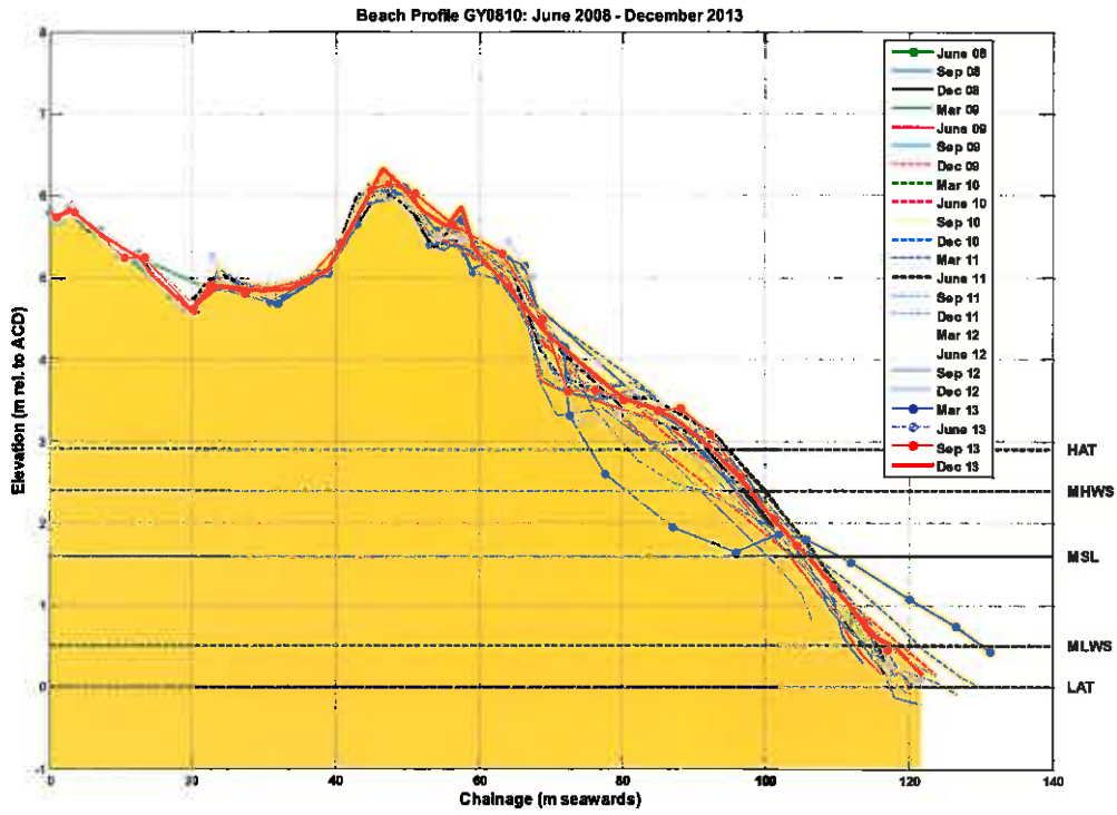
Figure B.11: Beach level surveys of profile GY0810
