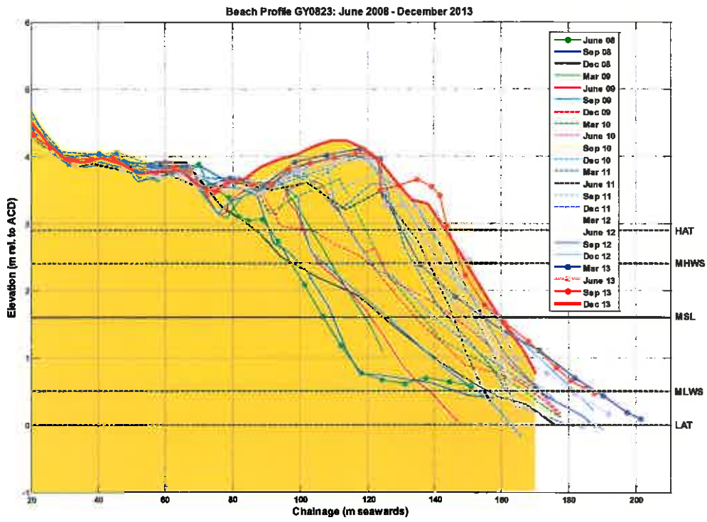
Figure B.19: Beach level surveys of profile GY0823
