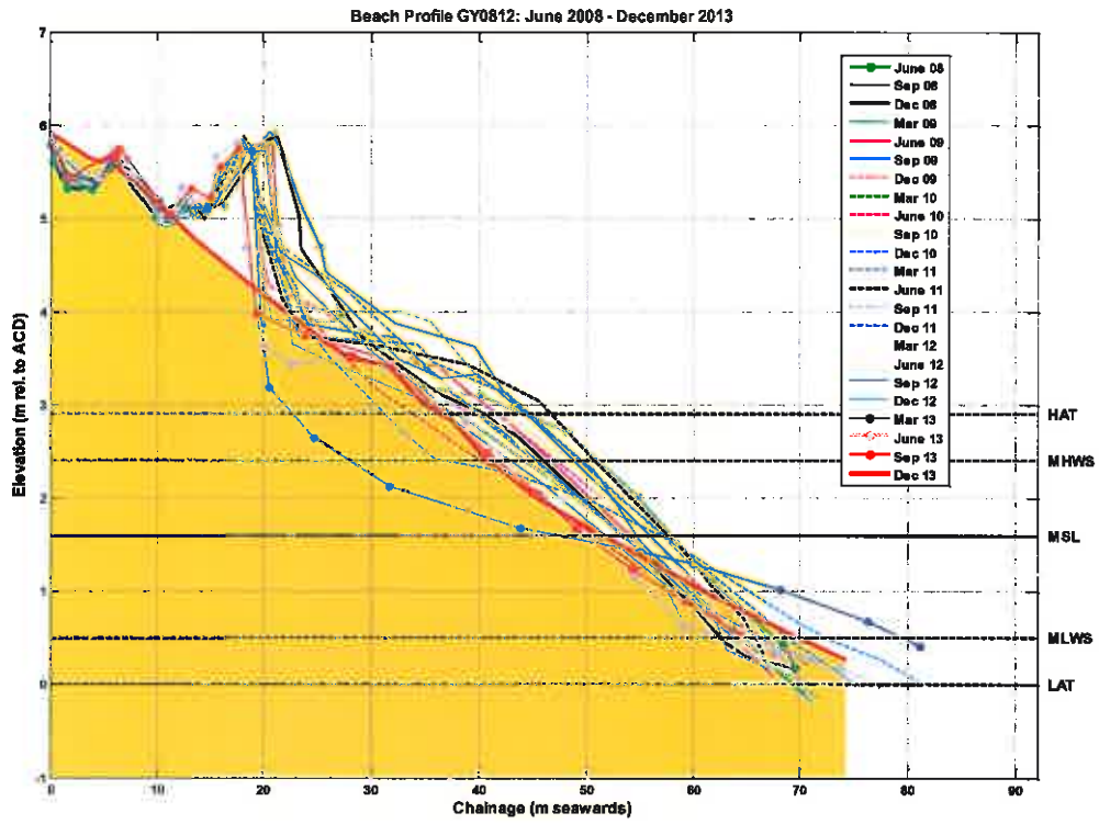
Figure B.13: Beach level surveys of profile GY0812
