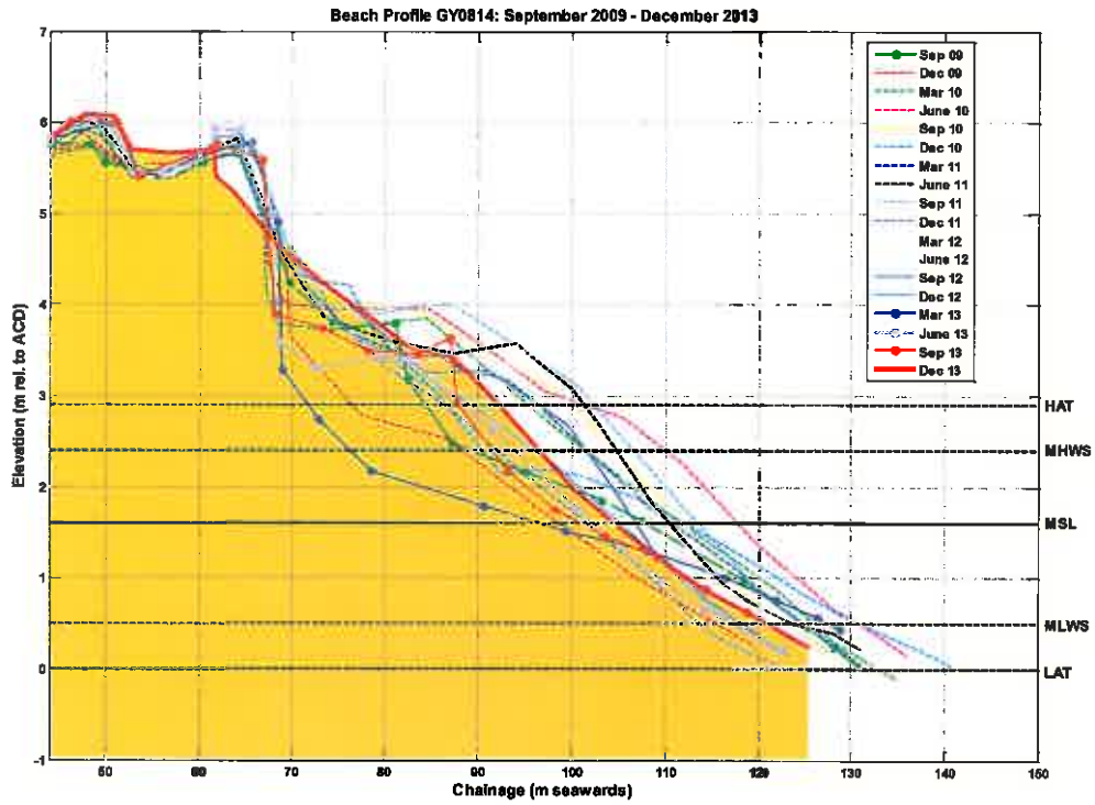
Figure B.15: Beach level surveys of profile GY0814
