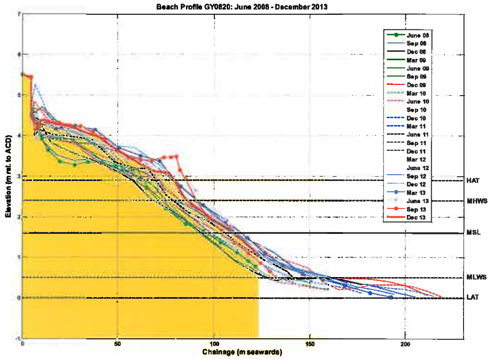
Figure B.16: Beach level surveys of profile GY0820
