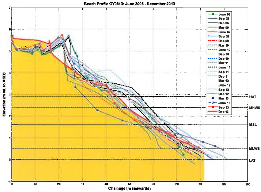
Figure B.14: Beach level surveys of profile GY0813
