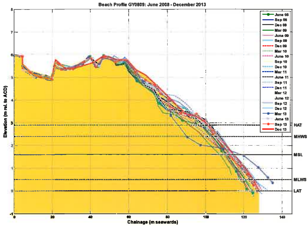
Figure B.10: Beach level surveys of profile GY0809
