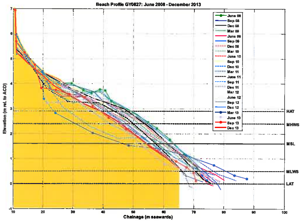
Figure B.23: Beach level surveys of profile GY0827
