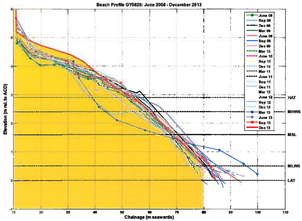
Figure B.22: Beach level surveys of profile GY0826
