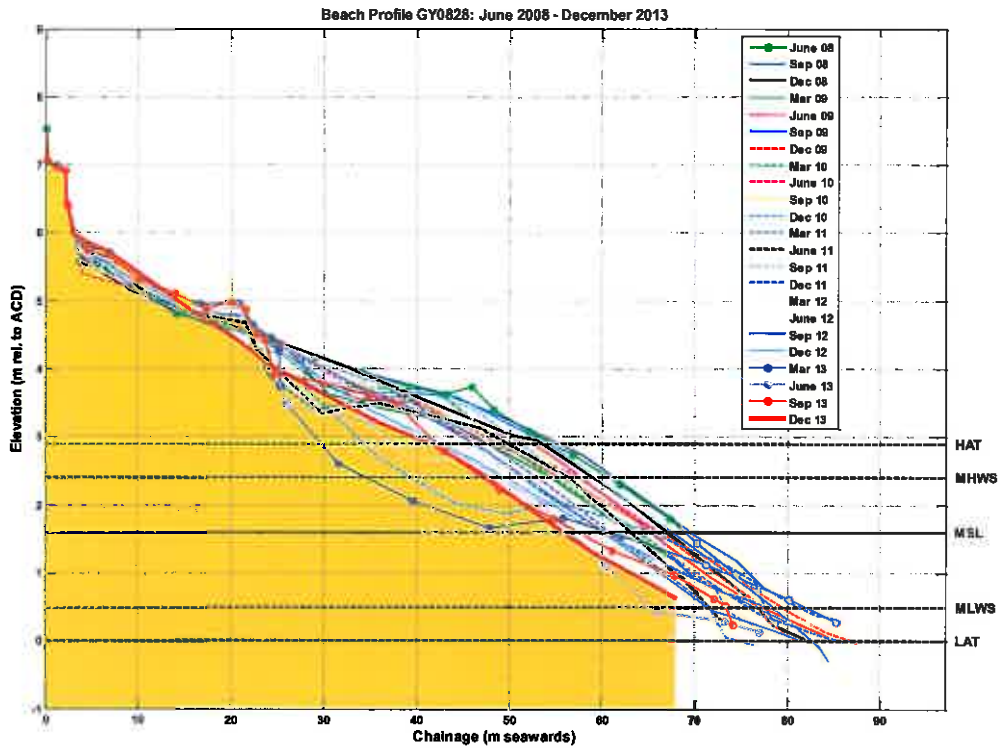
Figure B.24: Beach level surveys of profile GY0828
