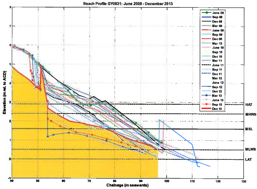
Figure B.27: Beach level surveys of profile GY0831
