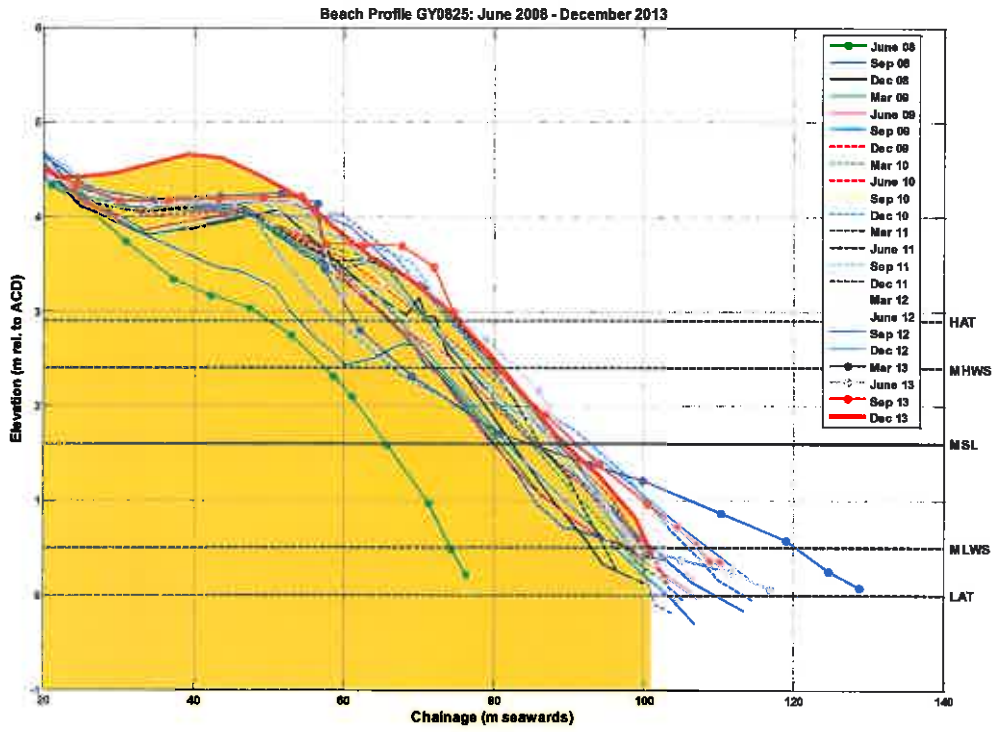
Figure B.21: Beach level surveys of profile GY0825
