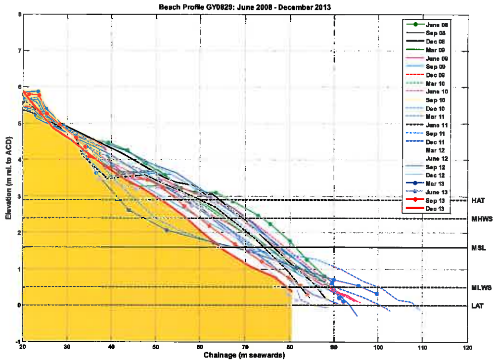
Figure B.25: Beach level surveys of profile GY0829
