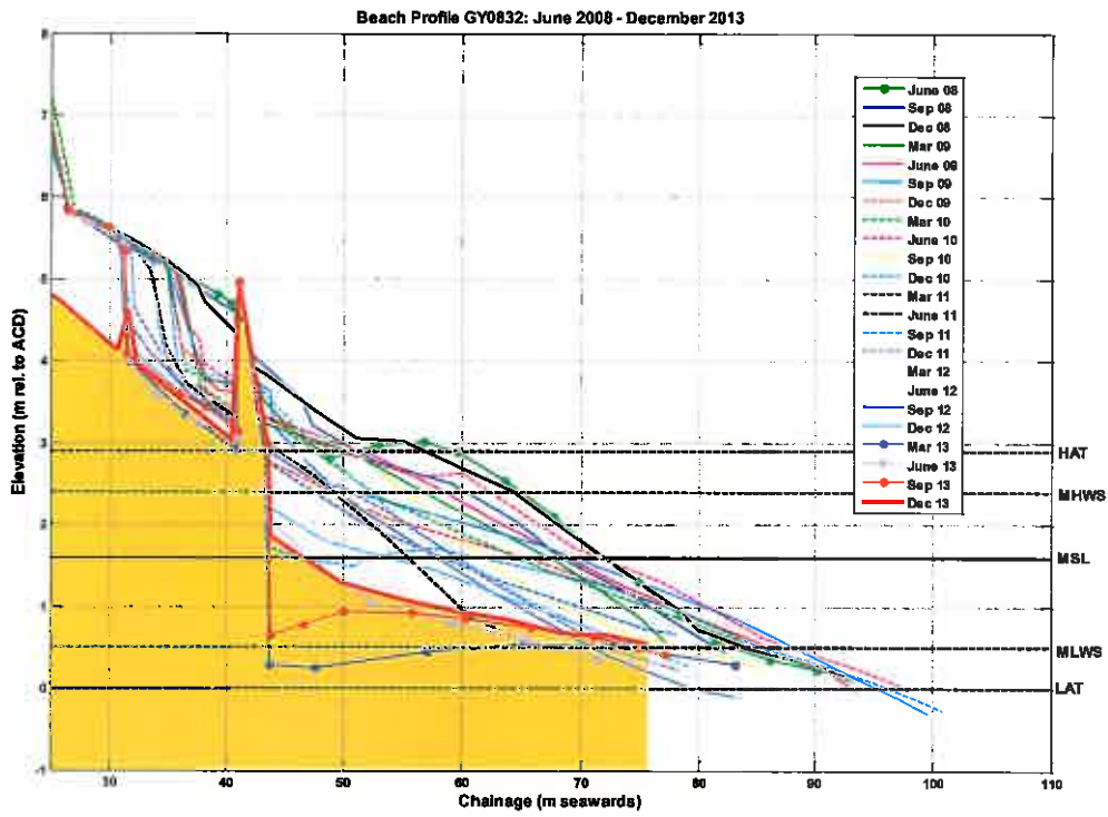
Figure B.28: Beach level surveys of profile GY0832
