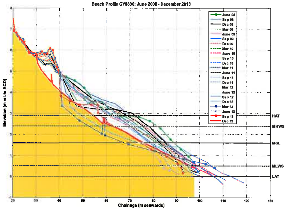
Figure B.26: Beach level surveys of profile GY0830
