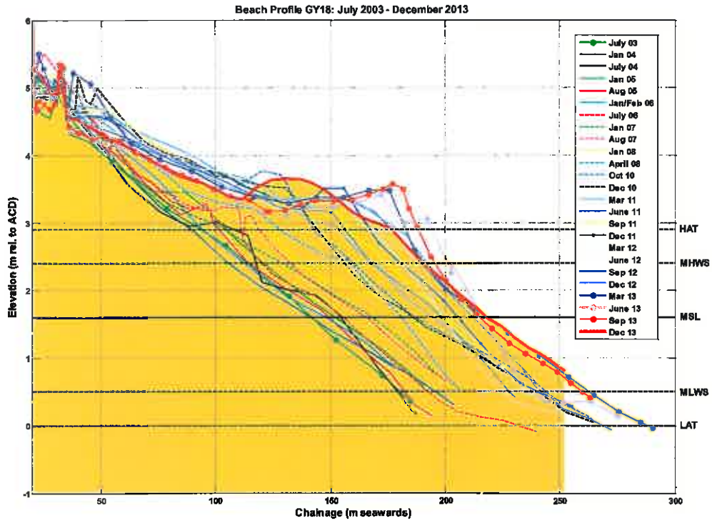
Figure B.38: Beach level surveys of profile GY18
