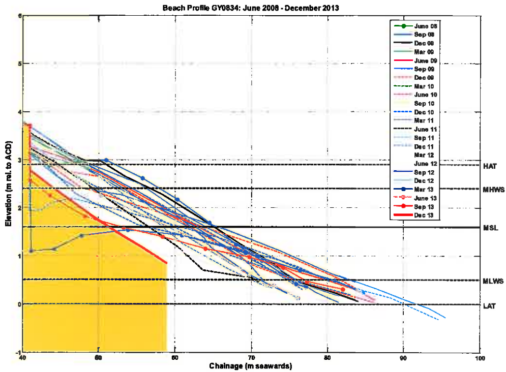
Figure B.30: Beach level surveys of profile GY0834
