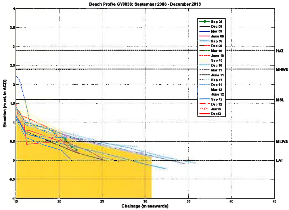
Figure B.34: Beach level surveys of profile GY0838
