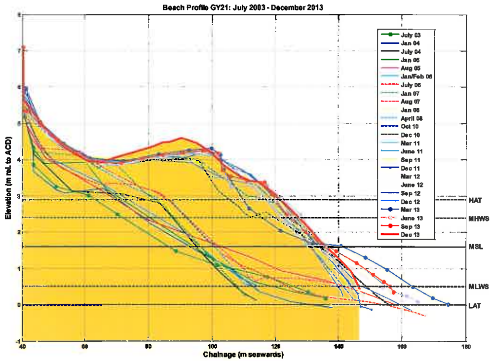
Figure B.41: Beach level surveys of profile GY21
