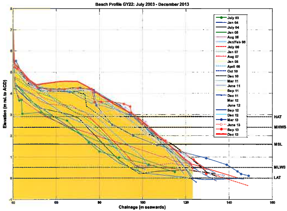
Figure B.42: Beach level surveys of profile GY22
