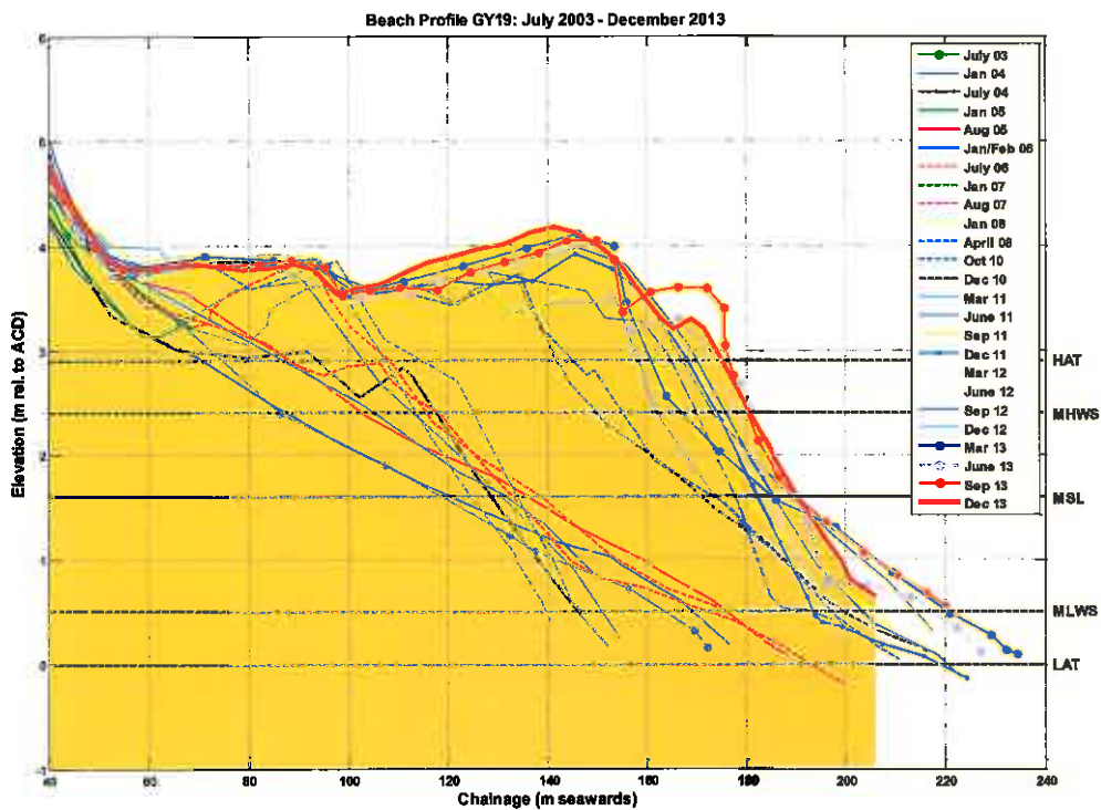
Figure B.39: Beach level surveys of profile GY19
