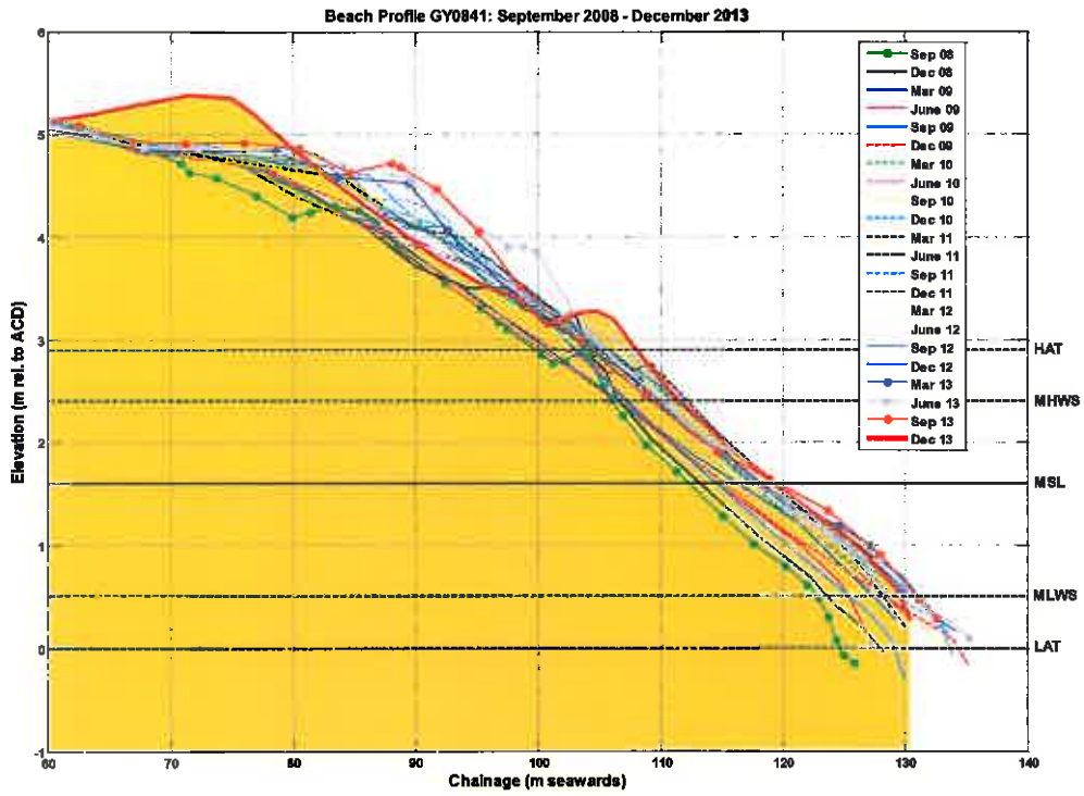
Figure B.37: Beach level surveys of profile GY0841
