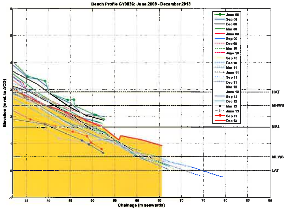
Figure B.32: Beach level surveys of profile GY0836
