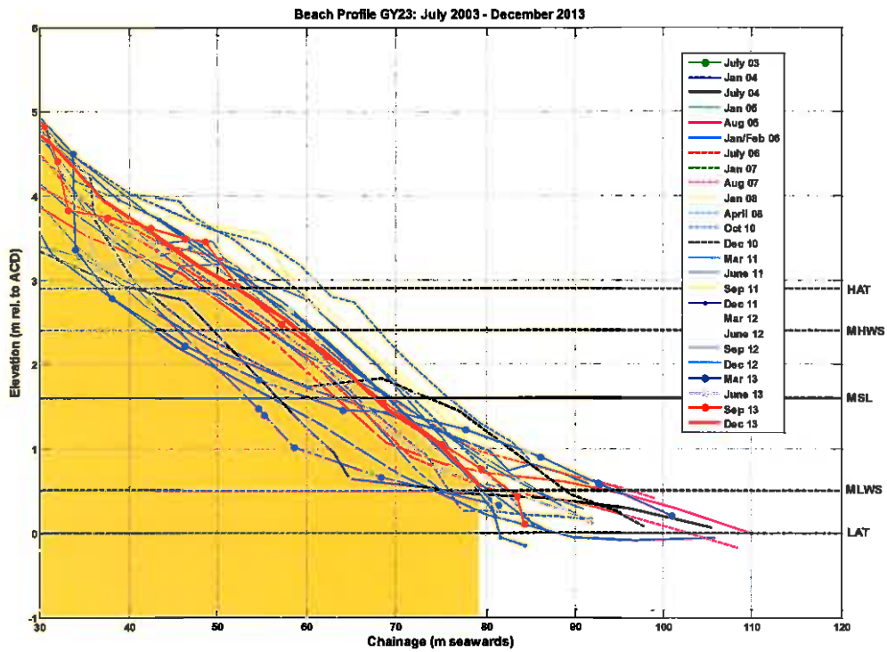
Figure B.43: Beach level surveys of profile GY23
