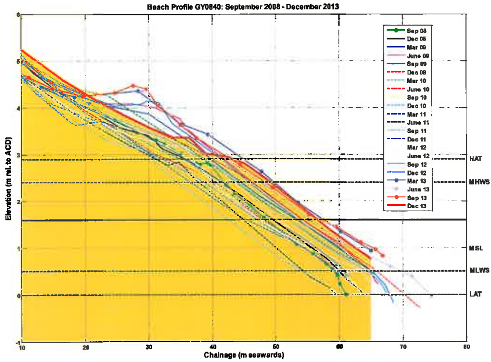
Figure B.36: Beach level surveys of profile GY0840
