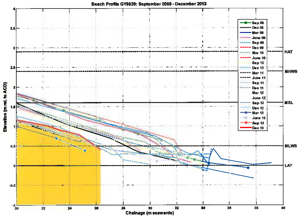
Figure B.35: Beach level surveys of profile GY0839
