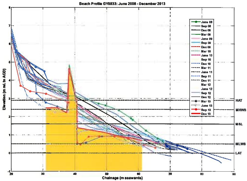
Figure B.29: Beach level surveys of profile GY0833
