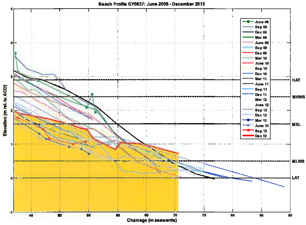
Figure B.33: Beach level surveys of profile GY0837
