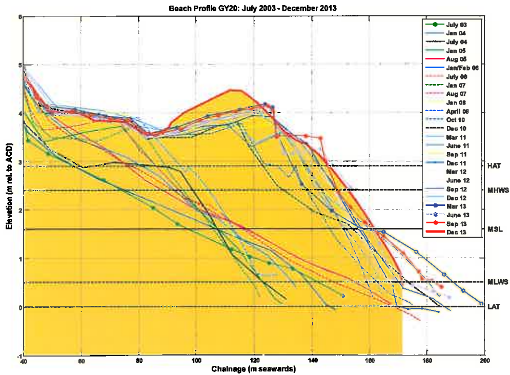
Figure B.40: Beach level surveys of profile GY20
