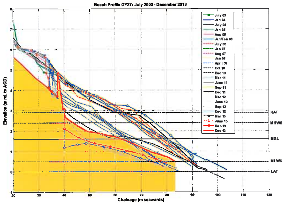
Figure B.47: Beach level surveys of profile GY27
