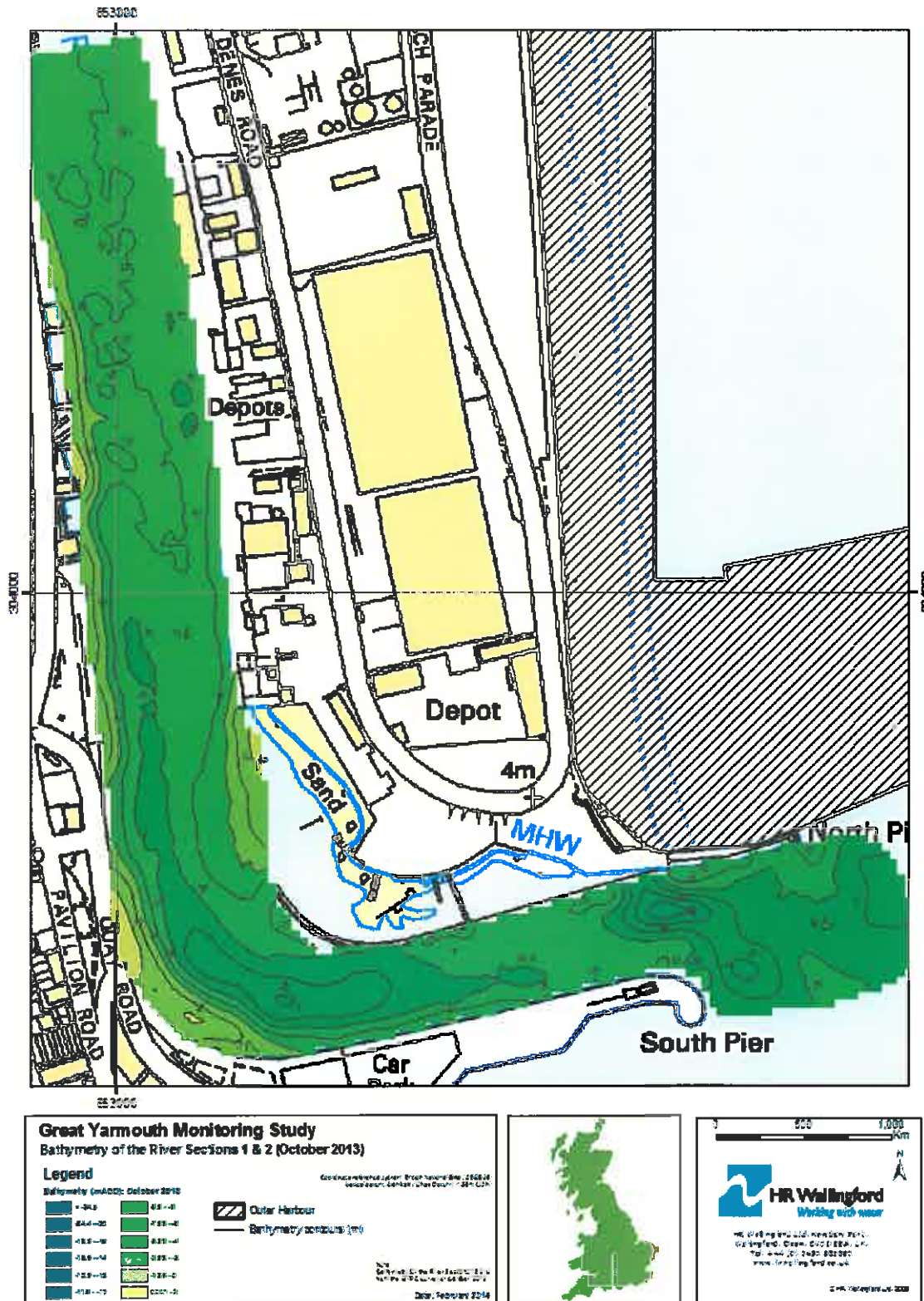
Figure B.54: Bathymetry of River Sections 1 & 2 surveyed in October 2013
