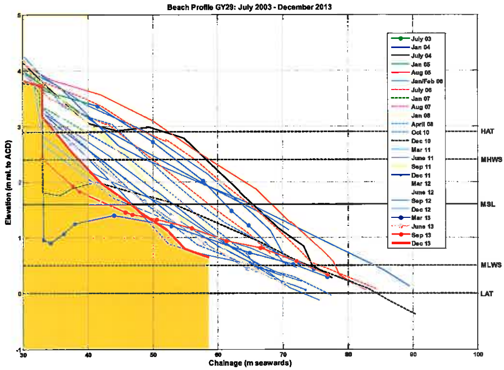
Figure B.49: Beach level surveys of profile GY29
