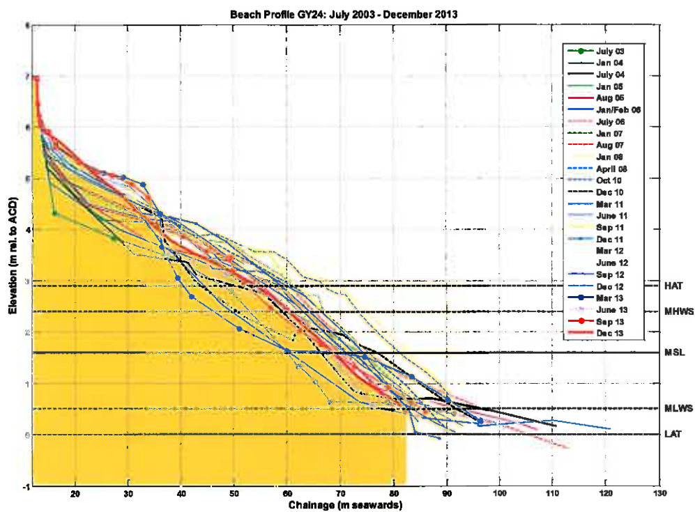
Figure B.44: Beach level surveys of profile GY24
