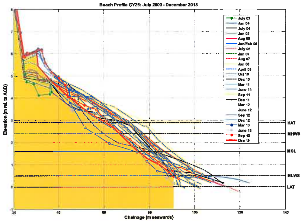
Figure B.45: Beach level surveys of profile GY25
