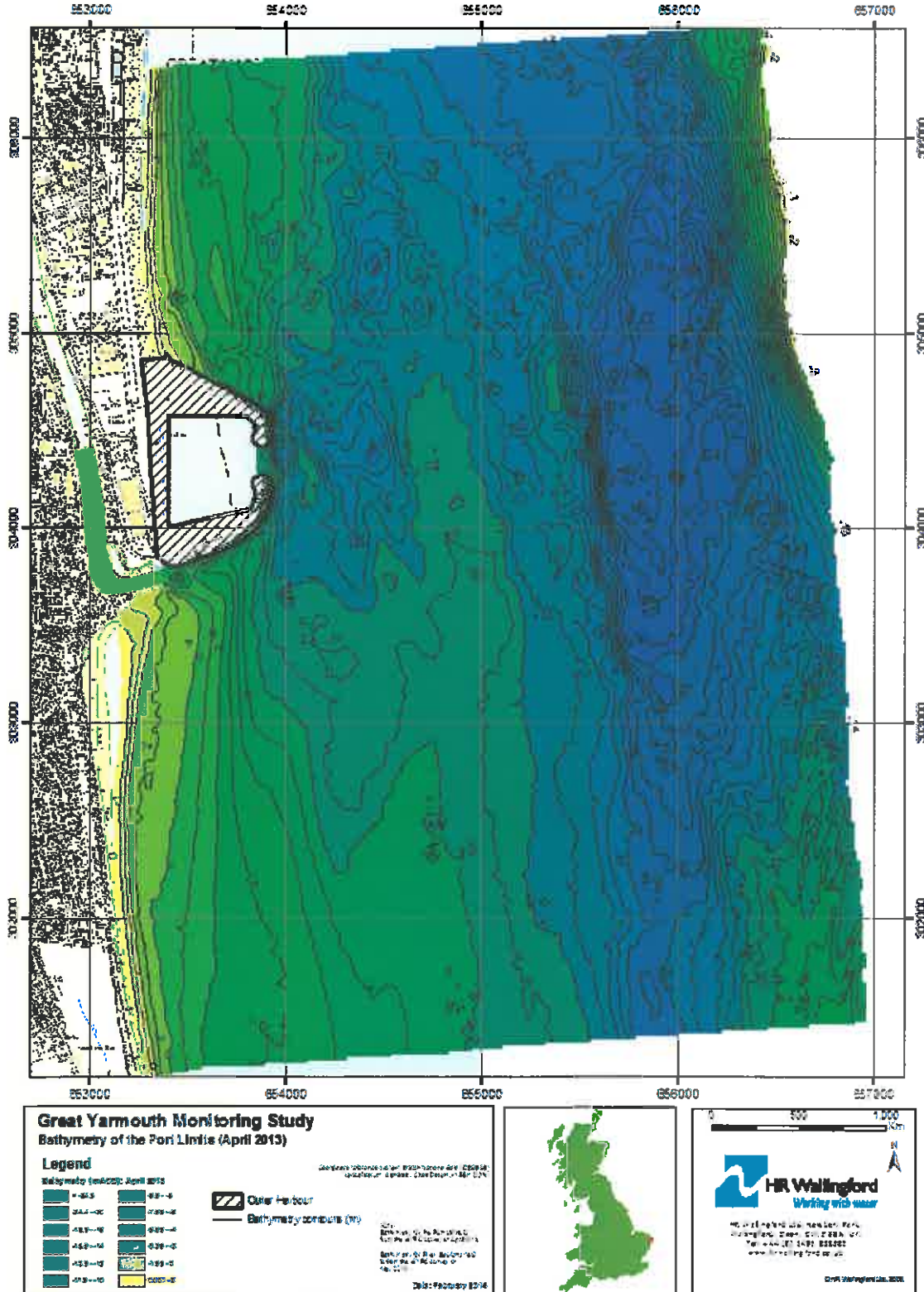
Figure B.51: Bathymetry of Port Limits Surveyed in April 2013
