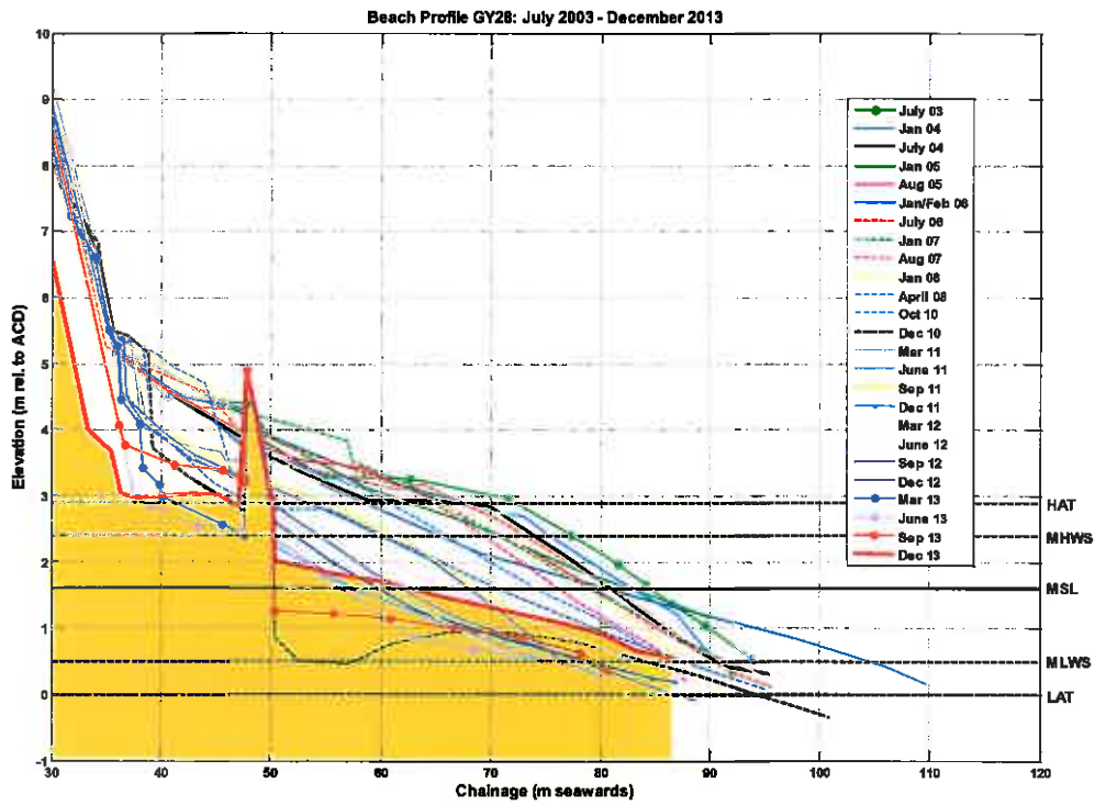
Figure B.48: Beach level surveys of profile GY28
