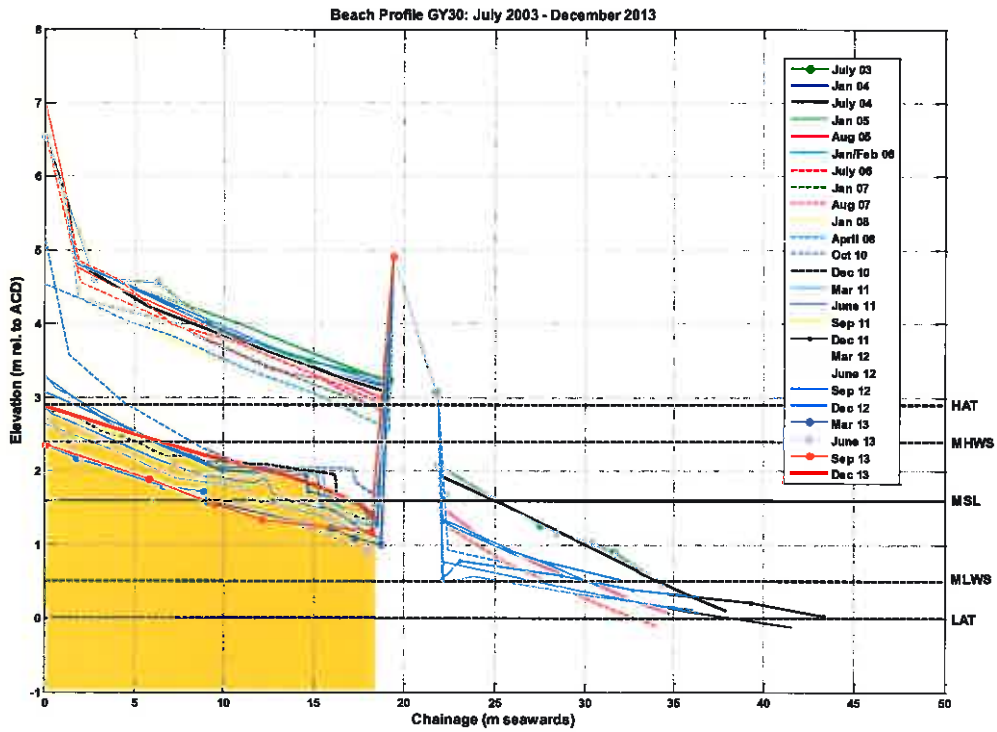
Figure B.50: Beach level surveys of profile GY30
