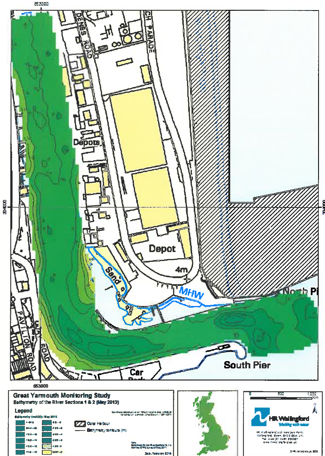
Figure B.53: Bathymetry of River Sections 1 & 2 surveyed in May 2013
