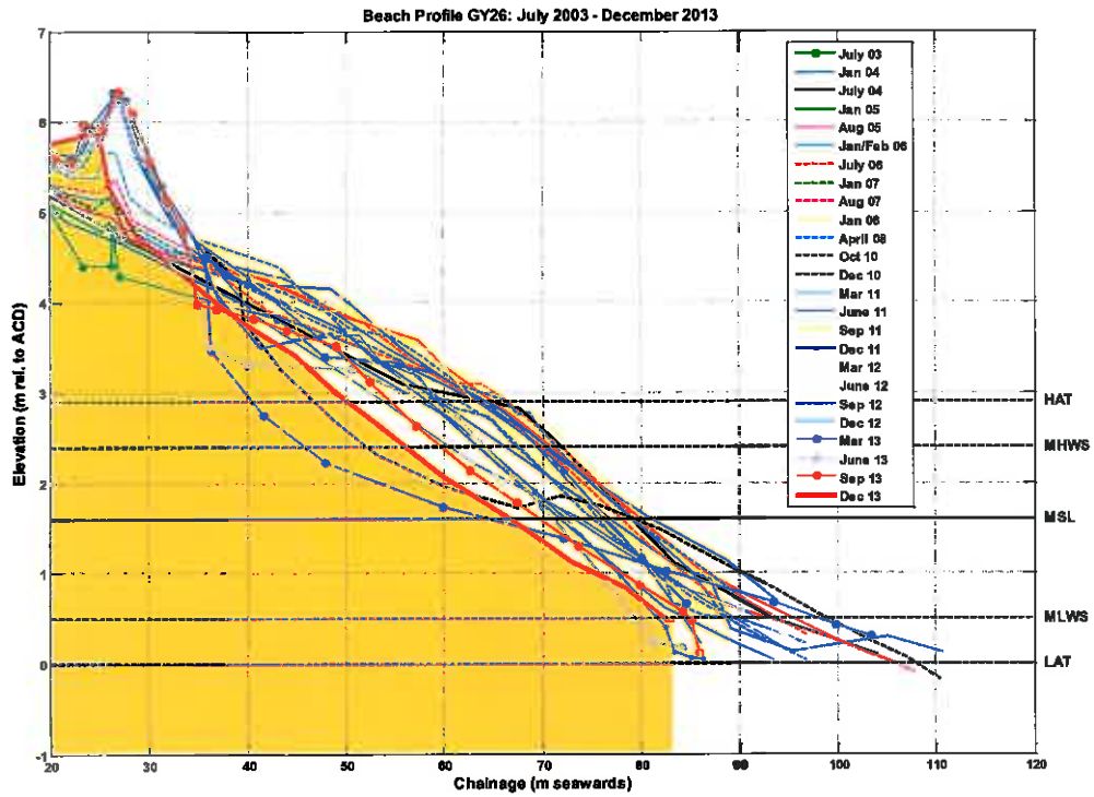
Figure B.46: Beach level surveys of profile GY26
