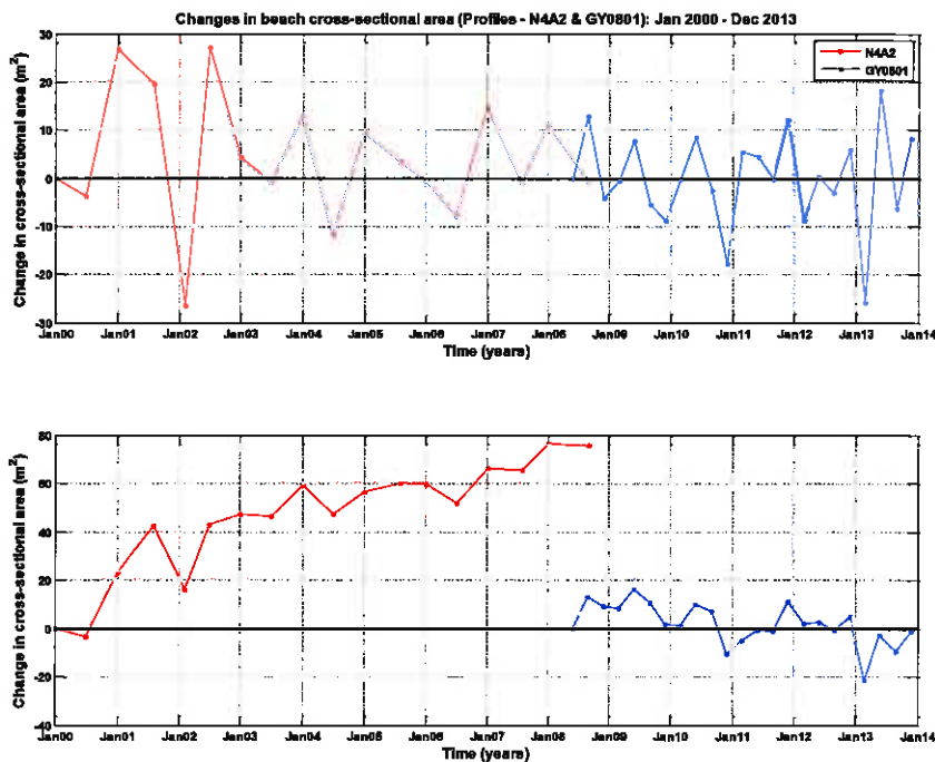
Figure B.56: (a) Time-series of 'successive' changes (i.e. change between consecutive surveys) in beach cross-sectional area at profiles N4A2 and GY0801. (b) Time-series of 'cumulative' changes (i.e. changes relative to first survey of the corresponding profile) in beach cross-sectional area at profiles N4A2 and GY0801.
