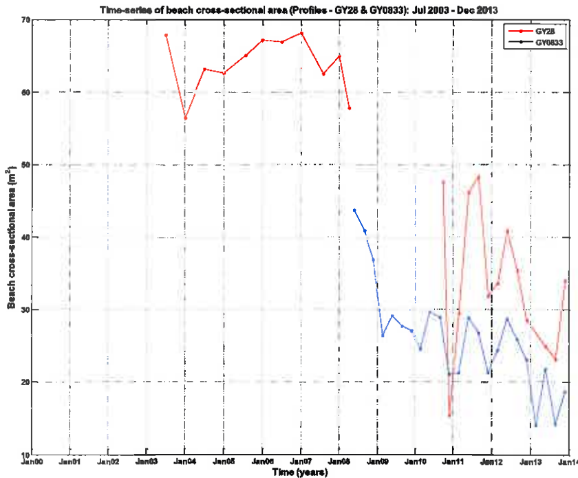
Figure B.71: Time-series of beach cross-sectional area at profiles GY28 and GY0833.
