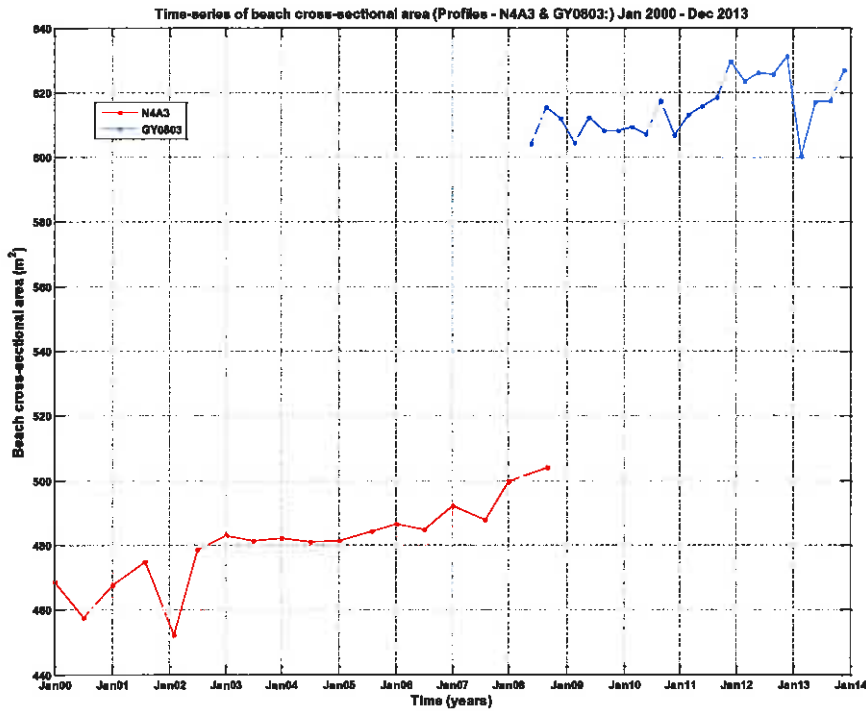
Figure B.57: Time-series of beach cross-sectional area at profiles N4A3 and GY0803.
