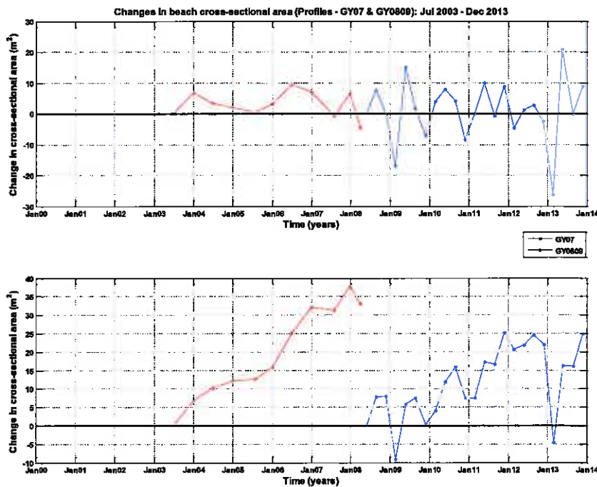
Figure B.62: (a) Time-series of 'successive' changes (i.e. change between consecutive surveys) in beach cross-sectional area at profiles GY07 and GY0809. (b) Time-series of 'cumulative' changes (i.e. changes relative to first survey of the corresponding profile) in beach cross-sectional area at profiles GY07 and GY0809.
