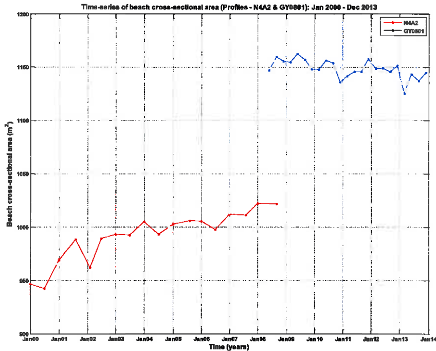
Figure B.55: Time-series of beach cross-sectional area at profiles N4A2 and GY0801.
