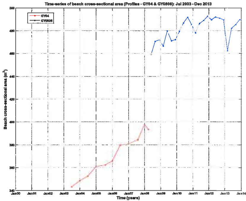
Figure B.59: Time-series of beach cross-sectional area at profiles GY04 and GY0806.
