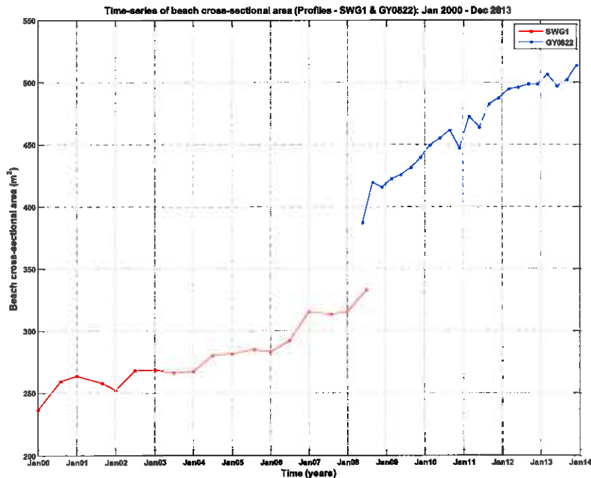
Figure B.67: Time-series of beach cross-sectional area at profiles SWG1 and GY0822.
