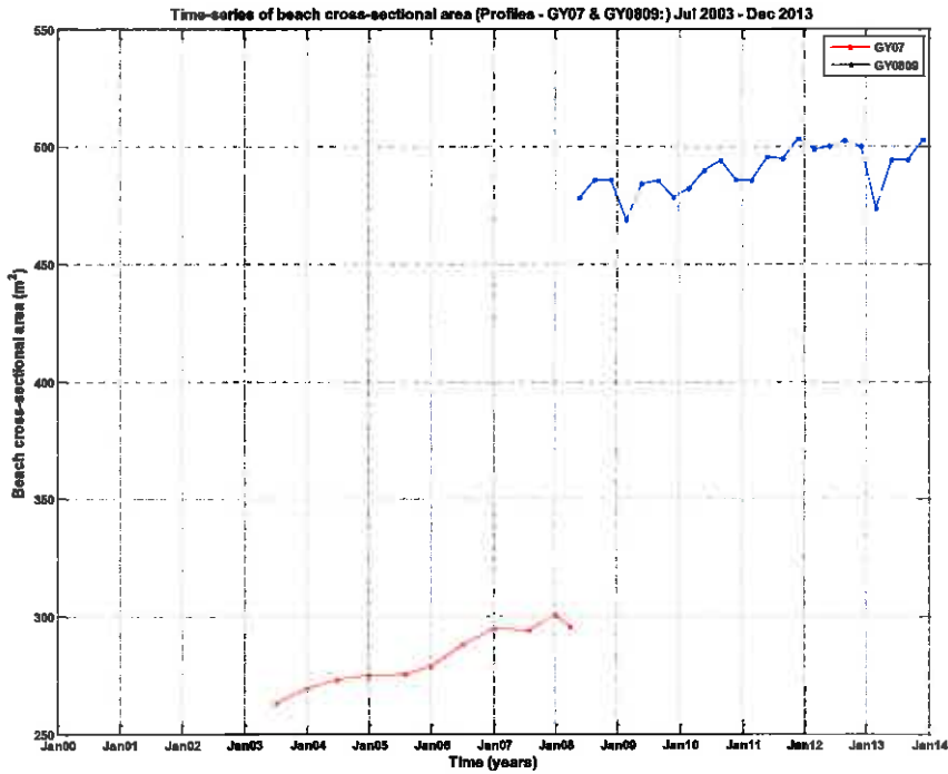
Figure B.61: Time-series of beach cross-sectional area at profiles GY07 and GY0809.
