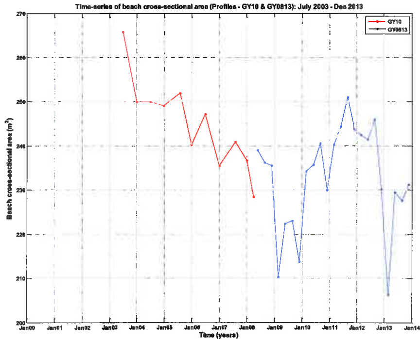
Figure B.63: Time-series of beach cross-sectional area at profiles GY10 and GY0813.
