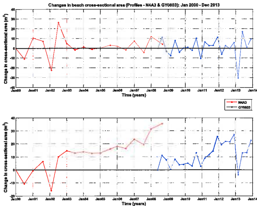
Figure B.58: (a) Time-series of 'successive' changes (i.e. change between consecutive surveys) in beach cross-sectional area at profiles N4A3 and GY0803. (b) Time-series of 'cumulative' changes (i.e. changes relative to first survey of the corresponding profile) in beach cross-sectional area at profiles N4A3 and GY0803.
