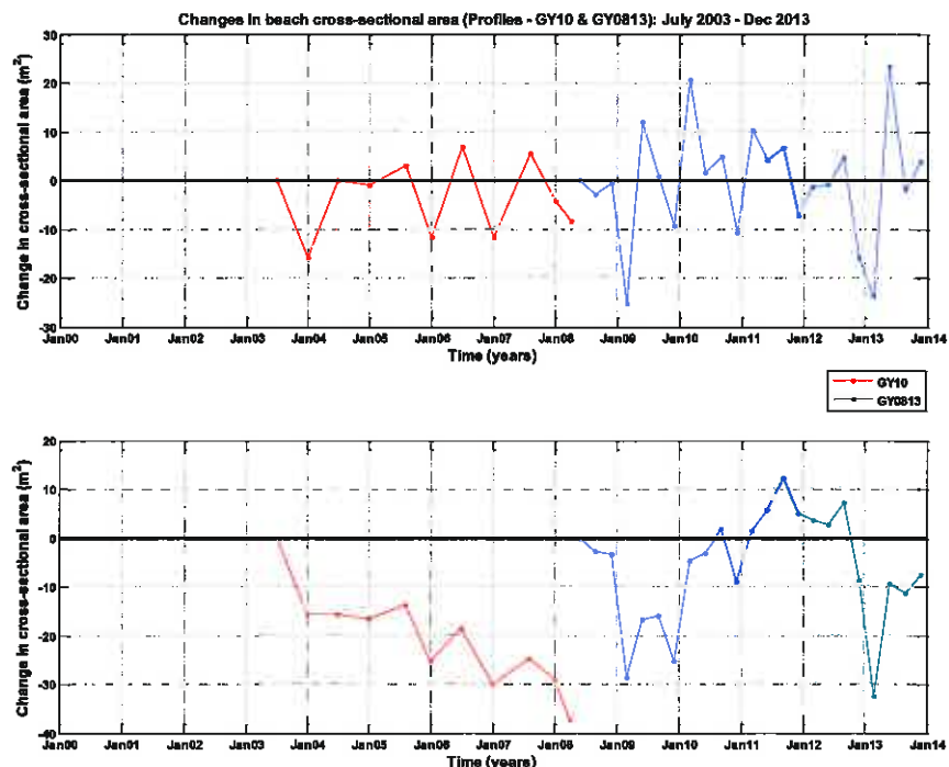
Figure B.64: (a) Time-series of 'successive' changes (i.e. change between consecutive surveys) in beach cross-sectional area at profiles GY10 and GY0813. (b) Time-series of 'cumulative' changes (i.e. changes relative to first survey of the corresponding profile) in beach cross-sectional area at profiles GY10 and GY0813.
