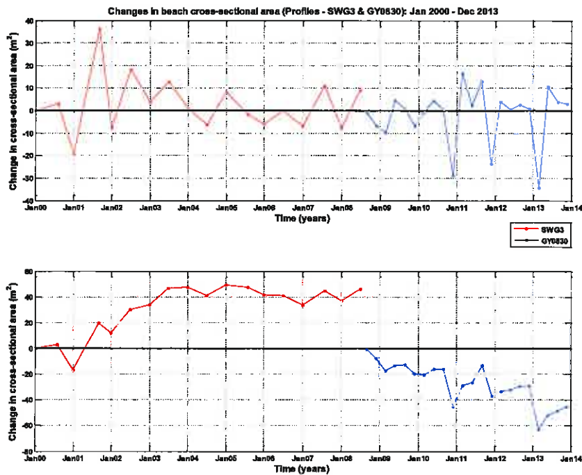
Figure B.70: (a) Time-series of 'successive' changes (i.e. change between consecutive surveys) in beach cross-sectional area at profiles SWG3 and GY0830. (b) Time-series of 'cumulative' changes (i.e. changes relative to first survey of the corresponding profile) in beach cross-sectional area at profiles SWG3 and GY0830.
