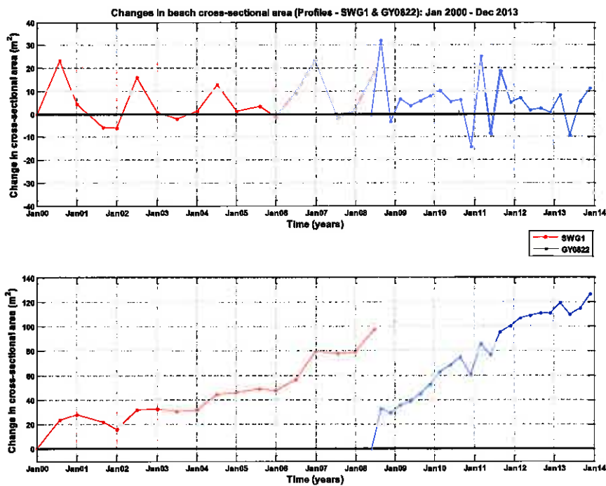
Figure B.68: (a) Time-series of 'successive' changes (i.e. change between consecutive surveys) in beach cross-sectional area at profiles SWG1 and GY0822. (b) Time-series of 'cumulative' changes (i.e. changes relative to first survey of the corresponding profile) in beach cross-sectional area at profiles SWG1 and GY0822.
