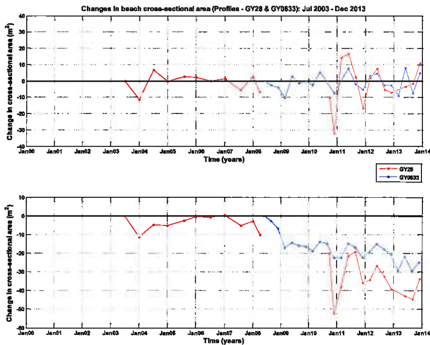
Figure B.72: (a) Time-series of 'successive' changes (i.e. change between consecutive surveys) in beach cross-sectional area at profiles GY28 and GY0833. (b) Time-series of 'cumulative' changes (i.e. changes relative to first survey of the corresponding profile) in beach cross-sectional area at profiles GY28 and GY0833.
