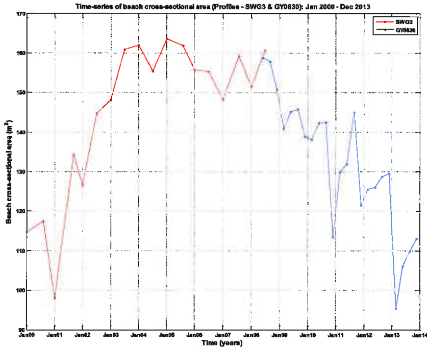
Figure B.69: Time-series of beach cross-sectional area at profiles SWG3 and GY0830.
