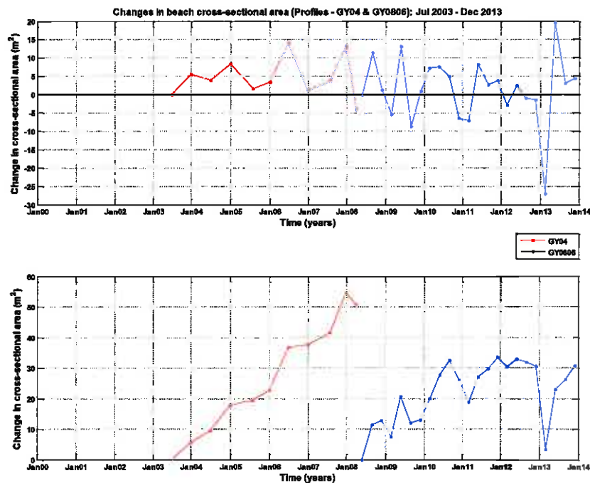
Figure B.60: (a) Time-series of 'successive' changes (i.e. change between consecutive surveys) in beach cross-sectional area at profiles GY04 and GY0806. (b) Time-series of 'cumulative' changes (i.e. changes relative to first survey of the corresponding profile) in beach cross-sectional area at profiles GY04 and GY0806.
