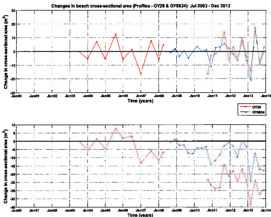
Figure B.74: (a) Time-series of 'successive' changes (i.e. change between consecutive surveys) in beach cross-sectional area at profiles GY29 and GY0834. (b) Time-series of 'cumulative' changes (i.e. changes relative to first survey of the corresponding profile) in beach cross-sectional area at profiles GY29 and GY0834.
