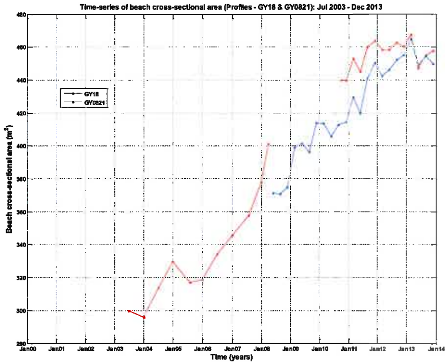
Figure B.65: Time-series of beach cross-sectional area at profiles GY18 and GY0821.
