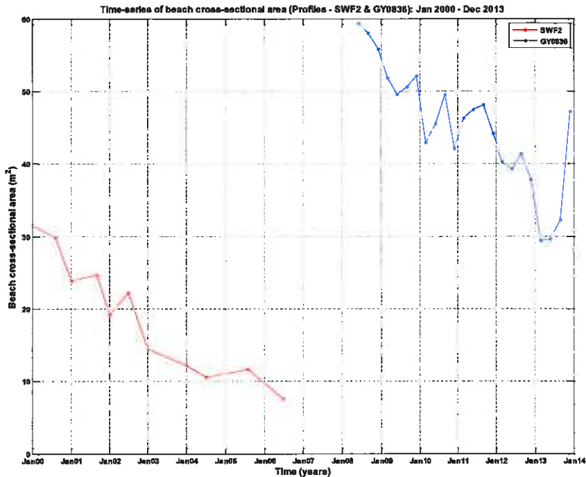
Figure B.75: Time-series of beach cross-sectional area at profiles SWF2 and GY0838.
