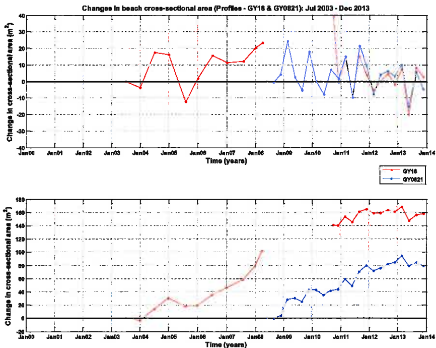
Figure B.66: (a) Time-series of 'successive' changes (i.e. change between consecutive surveys) in beach cross-sectional area at profiles GY18 and GY0821. (b) Time-series of 'cumulative' changes (i.e. changes relative to first survey of the corresponding profile) in beach cross-sectional area at profiles GY18 and GY0821.
