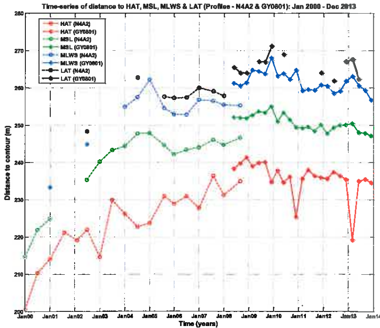
Figure B.81: Time-series of beach widths to HAT, MSL, MLWS and LAT at profiles N4A2 and GY0801.
