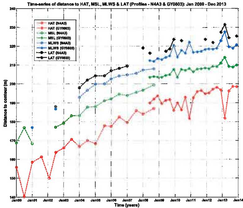
Figure B.83: Time-series of beach widths to HAT, MSL, MLWS and LAT at profiles N4A3 and GY0803.
