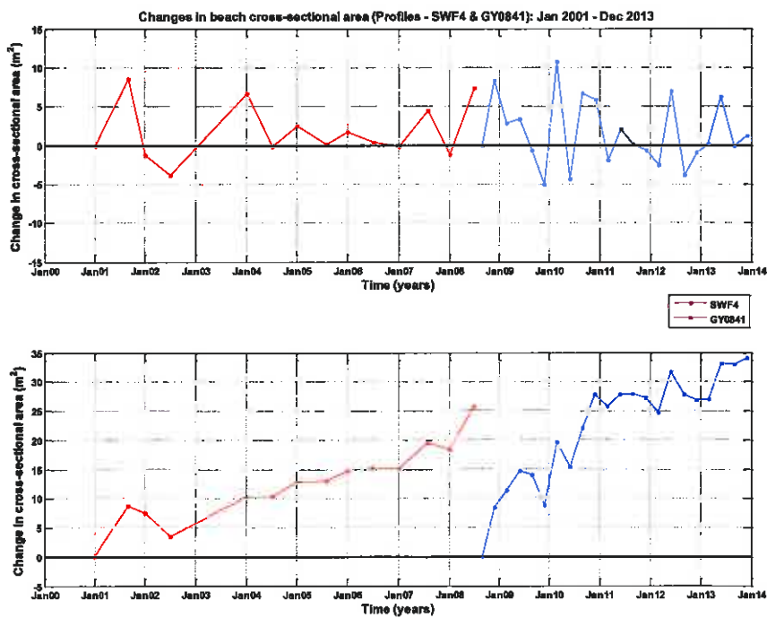
Figure B.80: (a) Time-series of 'successive' changes (i.e. change between consecutive surveys) in beach cross-sectional area at profiles SWF4 and GY0841. (b) Time-series of 'cumulative' changes (i.e. changes relative to first survey of the corresponding profile) in beach cross-sectional area at profiles SWF4 and GY0841.
