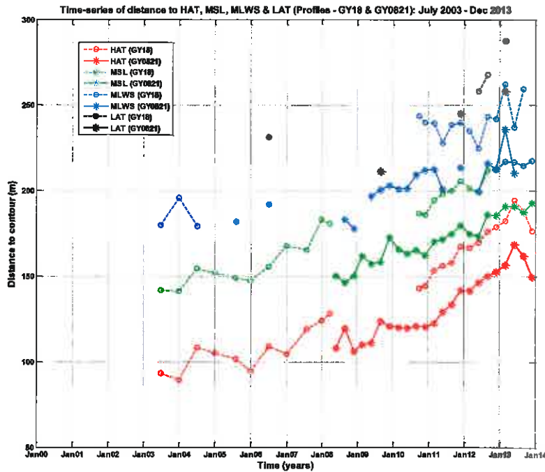
Figure B.91: Time-series of beach widths to HAT, MSL, MLWS and LAT at profiles GY18 and GY0821.
