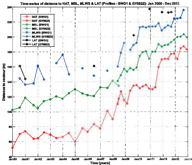
Figure B.93: Time-series of beach widths to HAT, MSL, MLWS and LAT at profiles SWG1 and GY0822.
