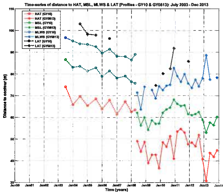
Figure B.89: Time-series of beach widths to HAT, MSL, MLWS and LAT at profiles GY10 and GY0813.
