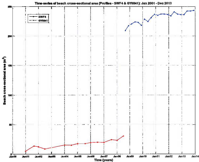
Figure B.79: Time-series of beach cross-sectional area at profiles SWF4 and GY0841.
