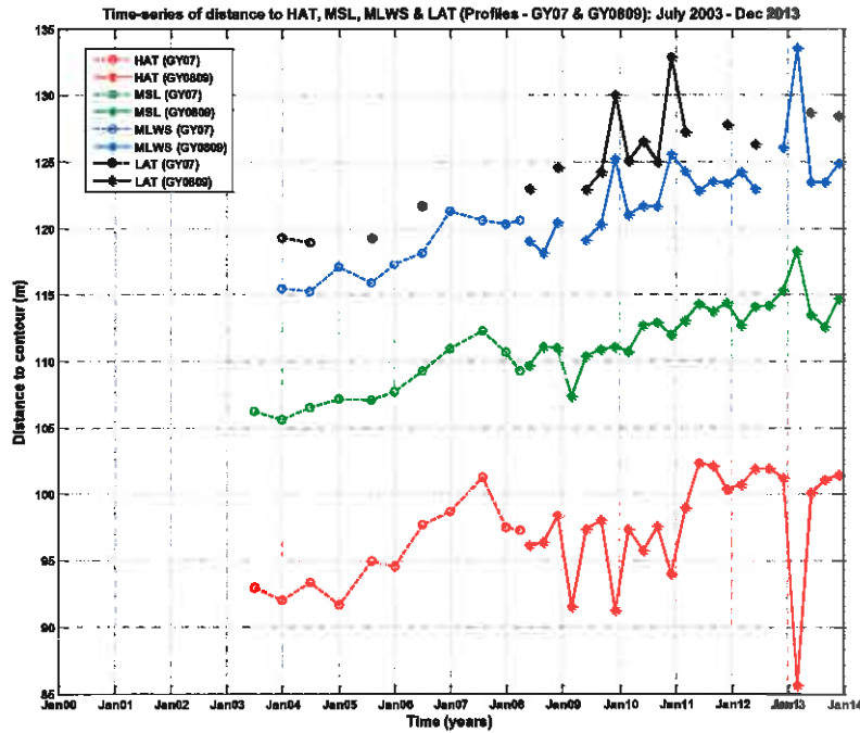
Figure B.87: Time-series of beach widths to HAT, MSL, MLWS and LAT at profiles GY07 and GY0809.
