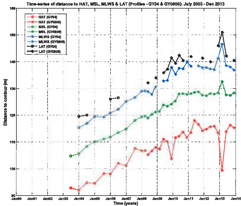
Figure B.85: Time-series of beach widths to HAT, MSL, MLWS and LAT at profiles GY04 and GY0808.
