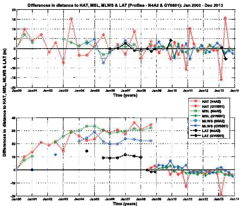
Figure B.82: (a) Time-series of 'successive' changes (i.e. change between consecutive surveys) in beach widths to HAT, MSL, MLWS and LAT at profiles N4A2 and GY0801. (b) Time-series of 'cumulative' changes (i.e. changes relative to first survey of the corresponding profile) in beach widths to HAT, MSL, MLWS and LAT at profiles N4A2 and GY0801.
