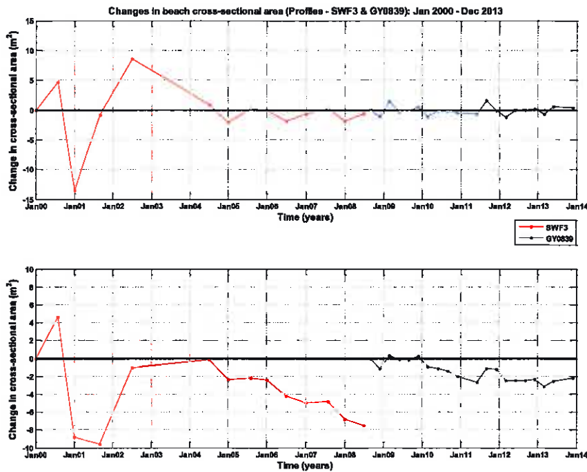
Figure B.78: (a) Time-series of 'successive' changes (i.e. change between consecutive surveys) in beach cross-sectional area at profiles SWF3 and GY0839. (b) Time-series of 'cumulative' changes (i.e. changes relative to first survey of the corresponding profile) in beach cross-sectional area at profiles SWF3 and GY0839.
