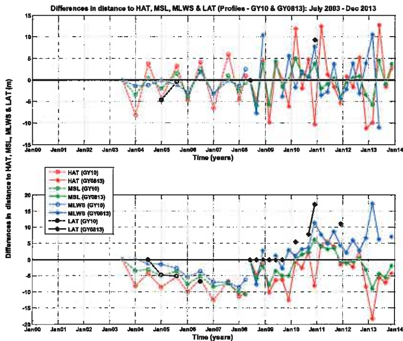
Figure B.90: (a) Time-series of 'successive' changes (i.e. change between consecutive surveys) in beach widths to HAT, MSL, MLWS and LAT at profiles GY10 and GY0813. (b) Time-series of 'cumulative' changes (i.e. changes relative to first survey of the corresponding profile) in beach widths to HAT, MSL, MLWS and LAT at profiles GY10 and GY0813.
