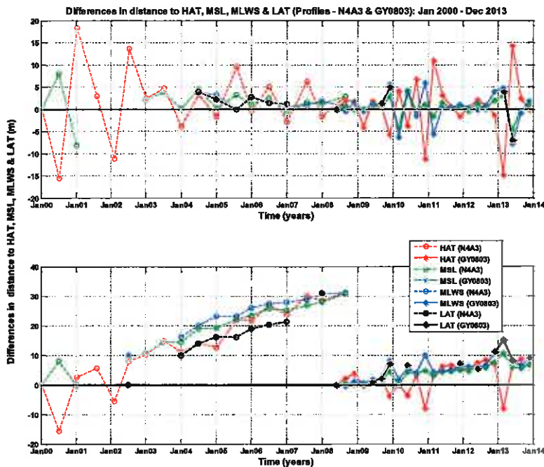
Figure B.84: (a) Time-series of 'successive' changes (i.e. change between consecutive surveys) in beach widths to HAT, MSL, MLWS and LAT at profiles N4A3 and GY0803. (b) Time-series of 'cumulative' changes (i.e. changes relative to first survey of the corresponding profile) in beach widths to HAT, MSL, MLWS and LAT at profiles N4A3 and GY0803.
