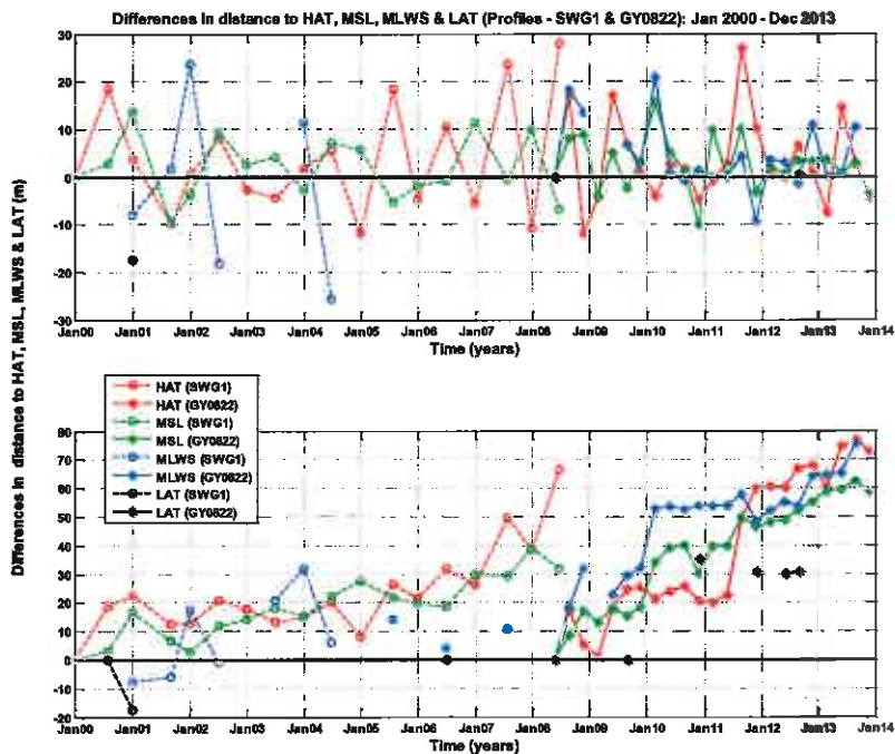
Figure B.94: (a) Time-series of 'successive' changes (i.e. change between consecutive surveys) in beach widths to HAT, MSL, MLWS and LAT at profiles SWG1 and GY0822. (b) Time-series of 'cumulative' changes (i.e. changes relative to first survey of the corresponding profile) in beach widths to HAT, MSL, MLWS and LAT at profiles SWG1 and GY0822.
