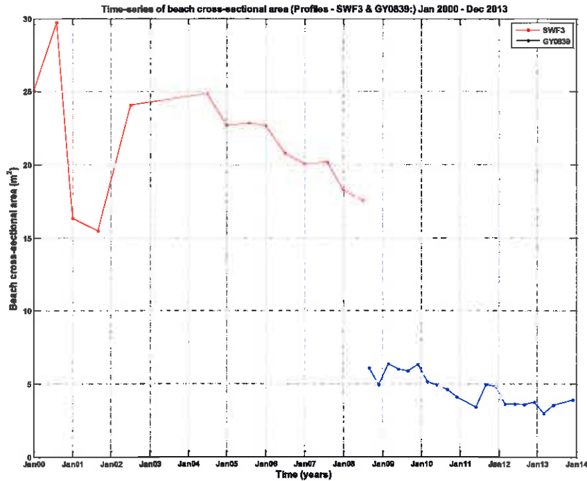
Figure B.77: Time-series of beach cross-sectional area at profiles SWF3 and GY0839.
