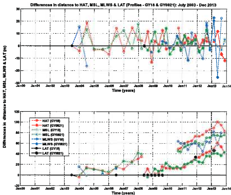
Figure B.92: (a) Time-series of 'successive' changes (i.e. change between consecutive surveys) in beach widths to HAT, MSL, MLWS and LAT at profiles GY18 and GY0821. (b) Time-series of 'cumulative' changes (i.e. changes relative to first survey of the corresponding profile) in beach widths to HAT, MSL, MLWS and LAT at profiles GY18 and GY0821.
