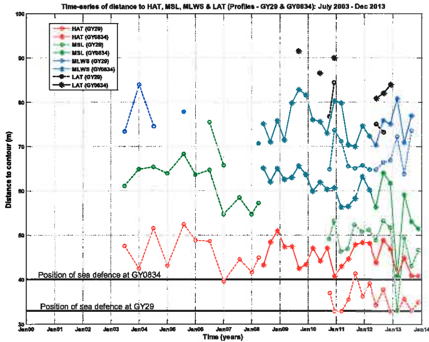
Figure B.99: Time-series of beach widths to HAT, MSL, MLWS and LAT at profiles GY29 and GY0834.
