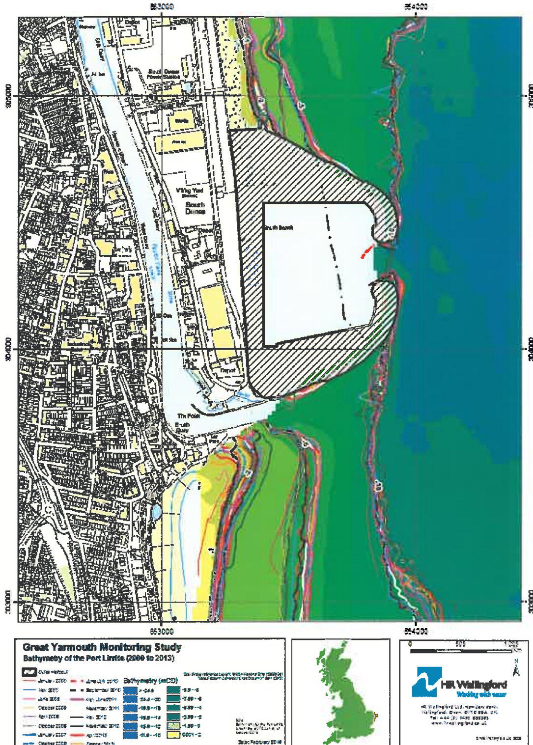
Figure B.108: Comparison of depth contours (-1m, -2m, -5m and -10m) within the Port Limits between January 2000 and October 2013
