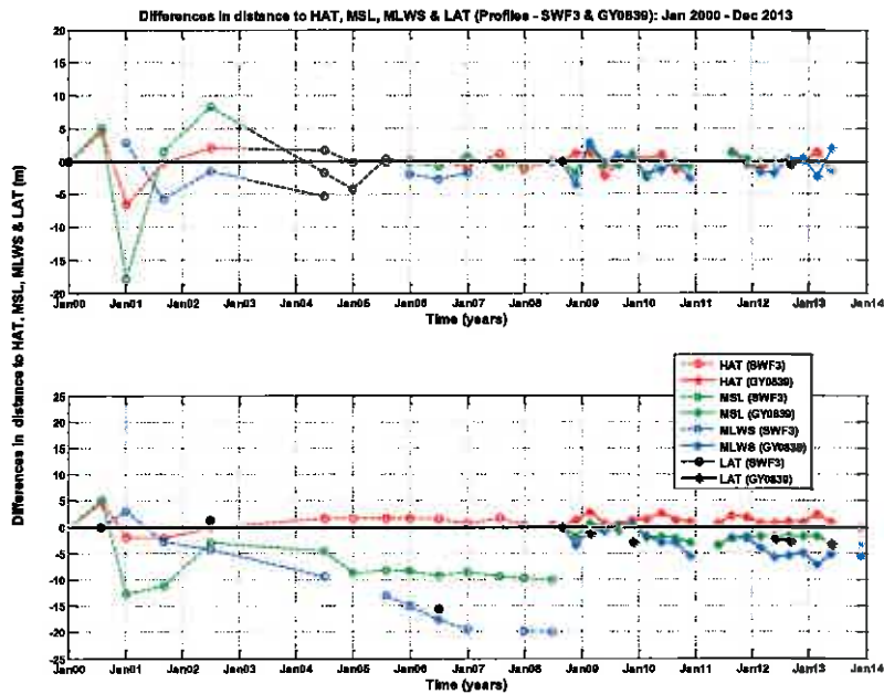
Figure B.104: (a) Time-series of 'successive' changes (i.e. change between consecutive surveys) in beach widths to HAT, MSL, MLWS and LAT at profiles SWF3 and GY0839. (b) Time-series of 'cumulative' changes (i.e. changes relative to first survey of the corresponding profile) in beach widths to HAT, MSL, MLWS and LAT at profiles SWF3 and GY0839.
