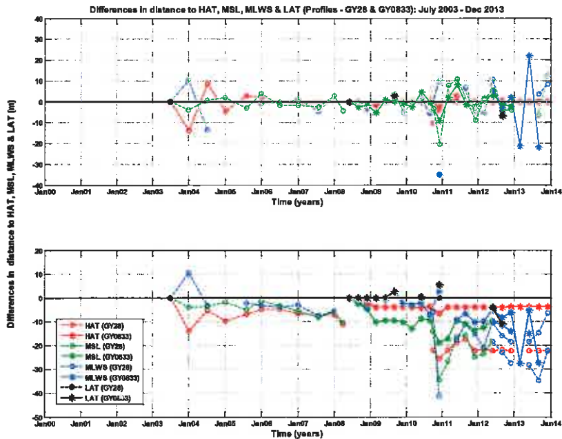
Figure B.98: (a) Time-series of 'successive' changes (i.e. change between consecutive surveys) in beach widths to HAT, MSL, MLWS and LAT at profiles GY28 and GY0833. (b) Time-series of 'cumulative' changes (i.e. changes relative to first survey of the corresponding profile) in beach widths to HAT, MSL, MLWS and LAT at profiles GY28 and GY0833.
