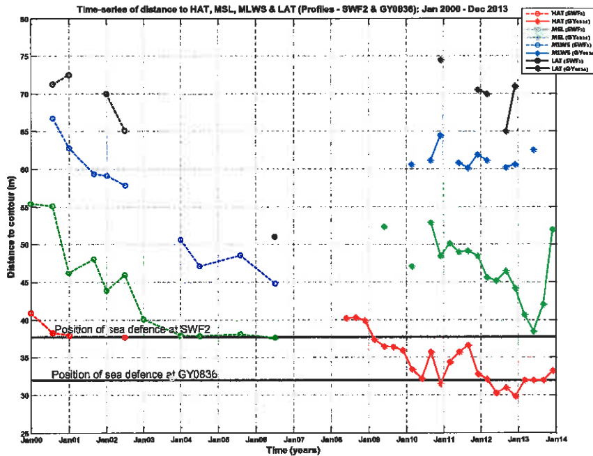
Figure B.101: Time-series of beach widths to HAT, MSL, MLWS and LAT at profiles SWF2 and GY0836.
