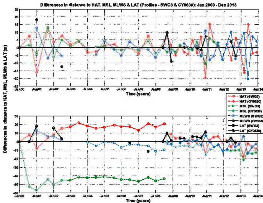
Figure B.96: (a) Time-series of 'successive' changes (i.e. change between consecutive surveys) in beach widths to HAT, MSL, MLWS and LAT at profiles SWG3 and GY0830. (b) Time-series of 'cumulative' changes (i.e. changes relative to first survey of the corresponding profile) in beach widths to HAT, MSL, MLWS and LAT at profiles SWG3 and GY0830.
