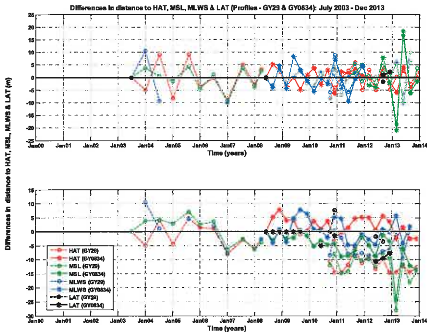
Figure B.100: (a) Time-series of 'successive' changes (i.e. change between consecutive surveys) in beach widths to HAT, MSL, MLWS and LAT at profiles GY29 and GY0834. (b) Time-series of 'cumulative' changes (i.e. changes relative to first survey of the corresponding profile) in beach widths to HAT, MSL, MLWS and LAT at profiles GY29 and GY0834.
