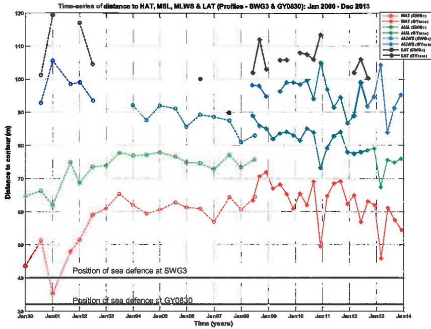
Figure B.95: Time-series of beach widths to HAT, MSL, MLWS and LAT at profiles SWG3 and GY0830.
