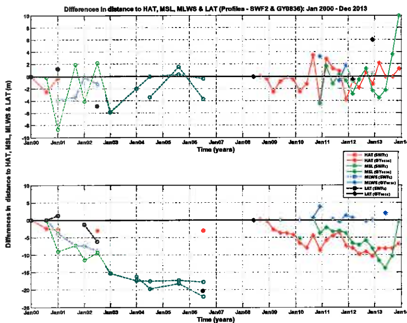
Figure B.102: (a) Time-series of 'successive' changes (i.e. change between consecutive surveys) in beach widths to HAT, MSL, MLWS and LAT at profiles SWF2 and GY0836. (b) Time-series of 'cumulative' changes (i.e. changes relative to first survey of the corresponding profile) in beach widths to HAT, MSL, MLWS and LAT at profiles SWF2 and GY0836.
