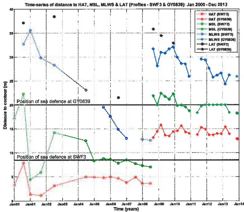
Figure B.103: Time-series of beach widths to HAT, MSL, MLWS and LAT at profiles SWF3 and GY0839.
