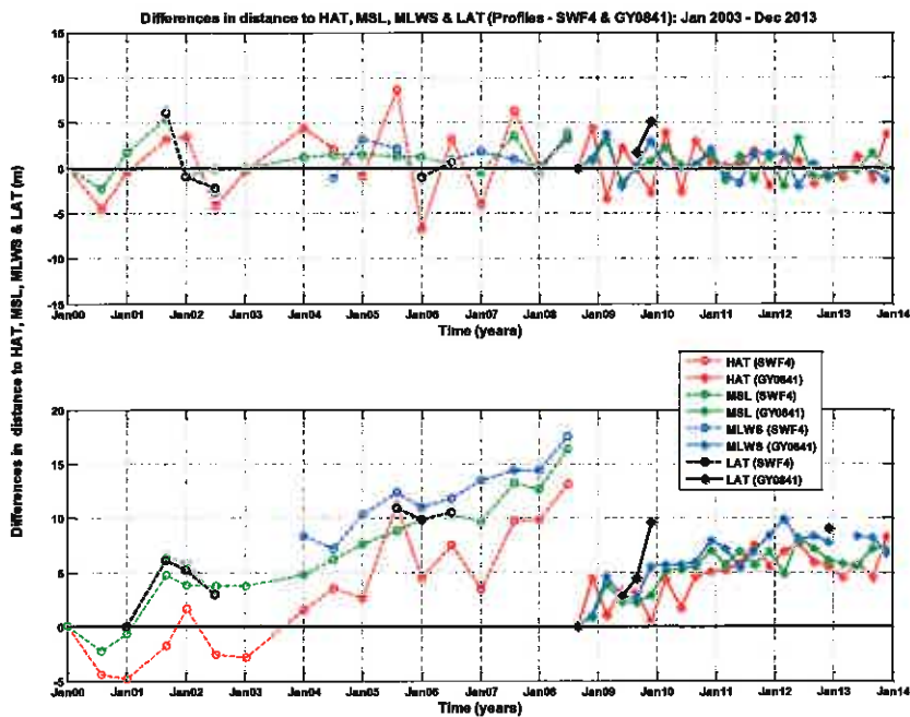
Figure B.106: (a) Time-series of 'successive' changes (i.e. change between consecutive surveys) in beach widths to HAT, MSL, MLWS and LAT at profiles SWF4 and GY0841. (b) Time-series of 'cumulative' changes (i.e. changes relative to first survey of the corresponding profile) in beach widths to HAT, MSL, MLWS and LAT at profiles SWF4 and GY0841.
