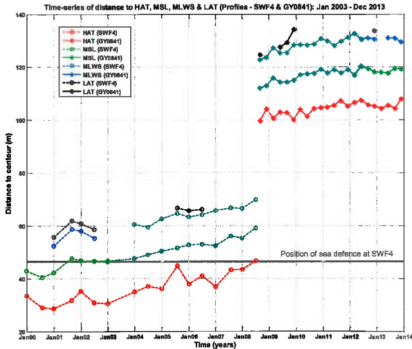
Figure B.105: Time-series of beach widths to HAT, MSL, MLWS and LAT at profiles SWF4 and GY0841.
