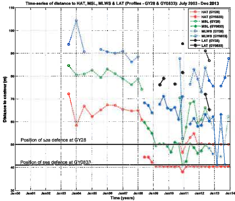
Figure B.97: Time-series of beach widths to HAT, MSL, MLWS and LAT at profiles GY28 and GY0833.
